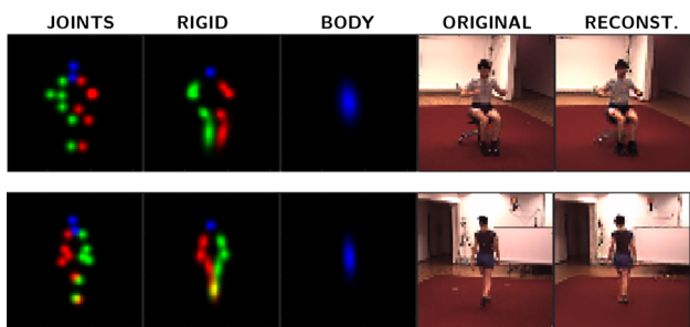
Fig. 14 Reconstructions on Human3.6M. From the left to right columns we have: joints, rigid parts and body heatmaps; original image and finally, the reconstructed image. In the heatmaps, right parts are shown in green, left parts in red and central parts in blue. Human3.6M images are 64 \times 64 pixels (Color figure online)
