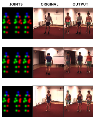
Fig. 17 Hallucinating multiple people on Human3.6M. The Conditional-DGPOSE model was trained with images containing only one person. The output images are generated keeping the appearance of the original images but conditioned to the manipulated heatmap pose representation (left). Heatmaps of rigid parts and whole body are not shown for simplicity
