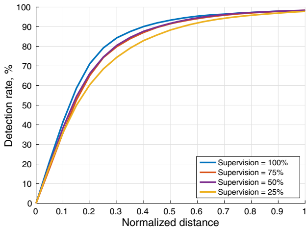
Fig. 28 Accuracy of Poses on Human3.6M. Quantitative evaluations of Semi-DGPos for different levels of supervision using the PCK scores. Note that, even with 25% supervision, our Semi-DGPos obtains 88.35% PCK score, normalised at 0.5
