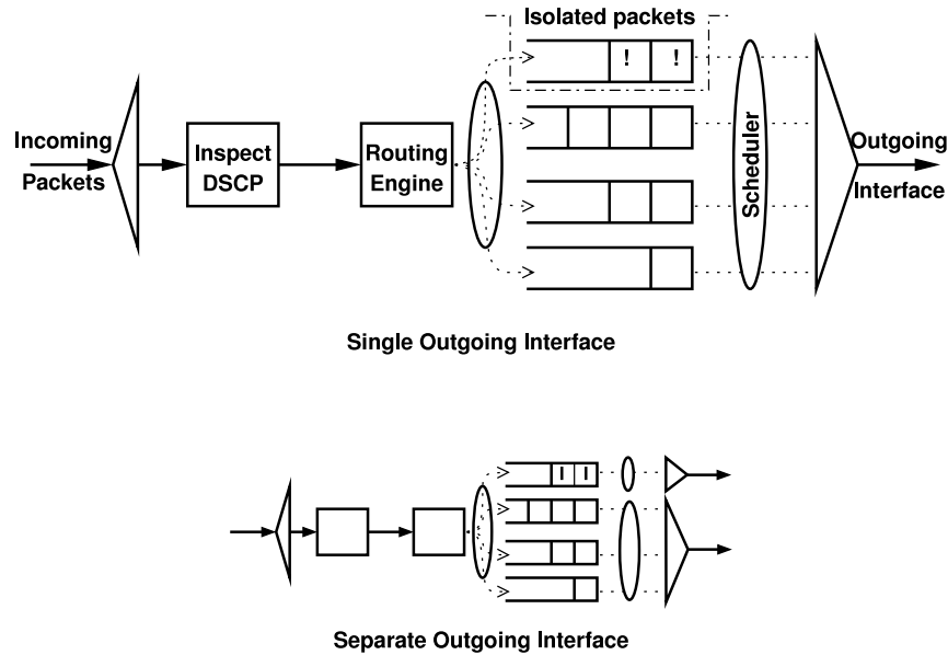
Figure 1. DSCP-based isolation inside a router.
