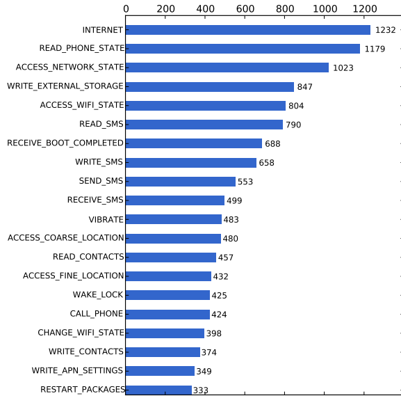
(a) Top 20 Permissions Requested By 1260 Malware Samples
