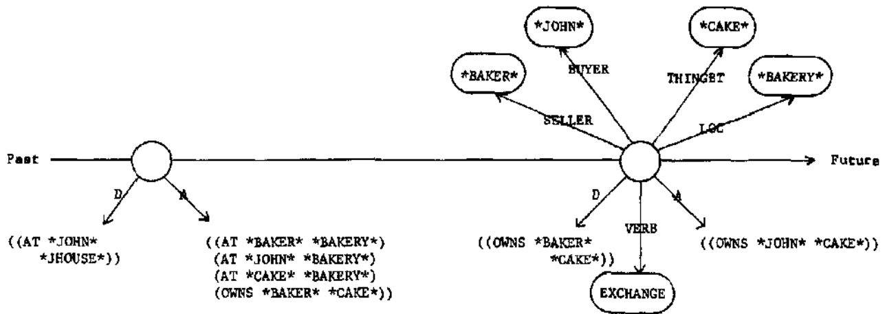
FIGURE 5 Time Line Nodes Created by an Event Procedure
