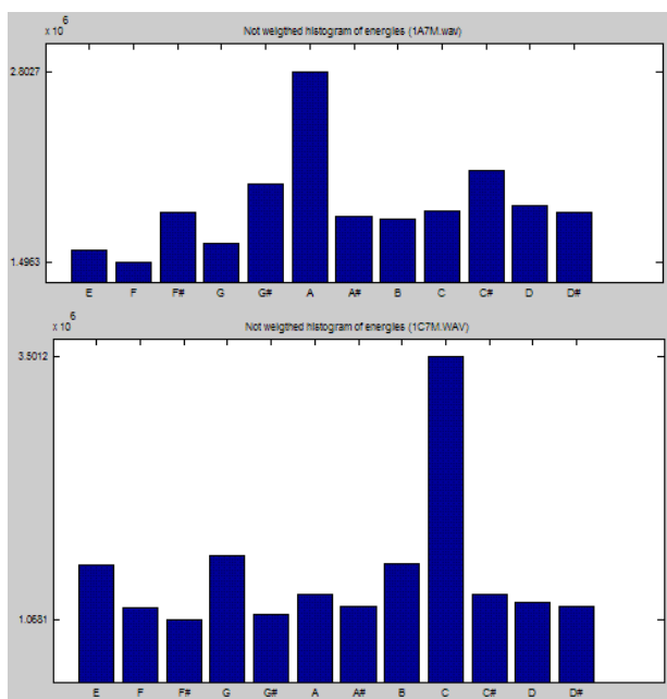
Figure 1. Examples of PCPs for a Amaj7 (above) and a Cmaj7 (below).
