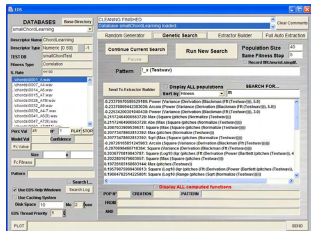
Figure 2. EDS main interface.
