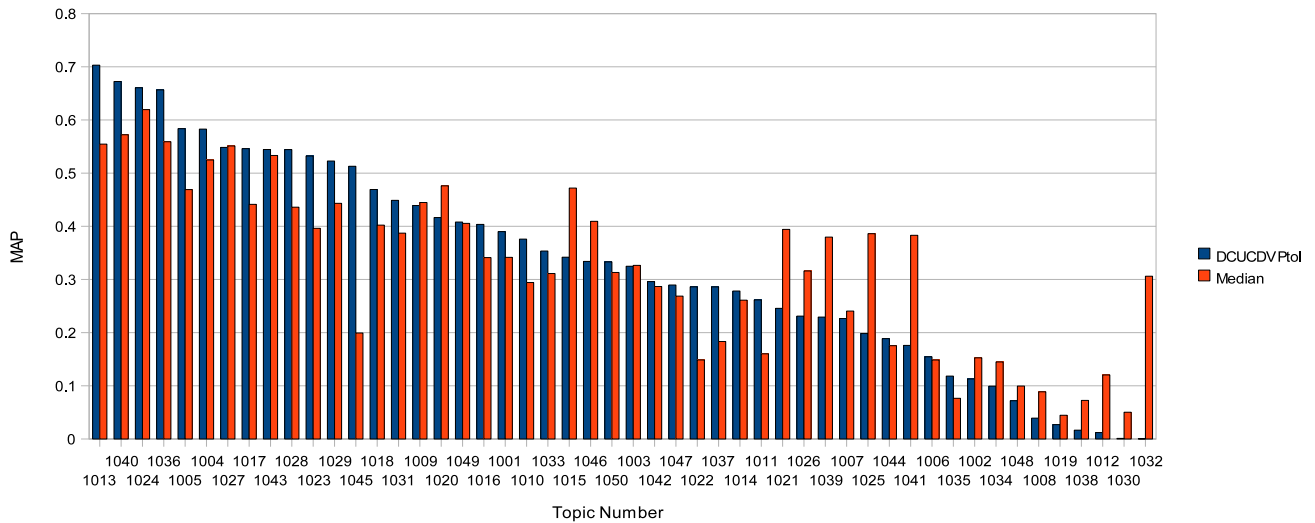
Figure 2: Per-topic MAP for the best-performing opinion run based on a non-distributed baseline, DCU’s topic only baseline.
