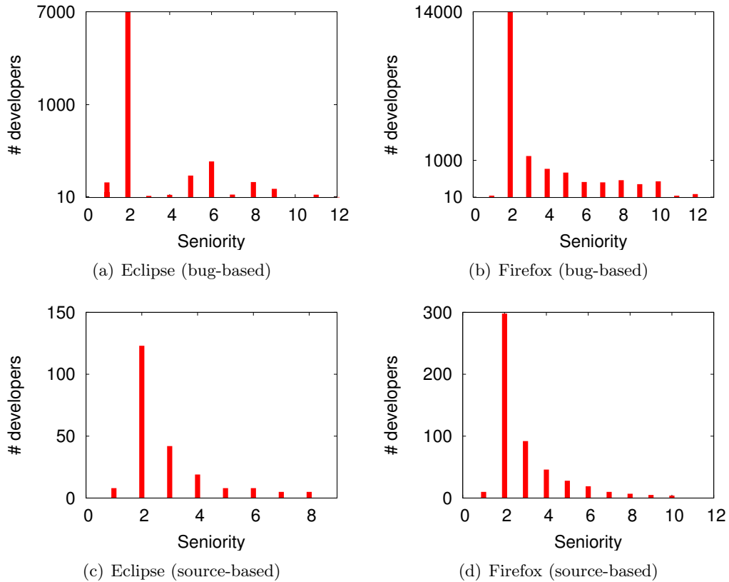
Figure 6.2: Bugfix-induced and source code-induced seniority.
