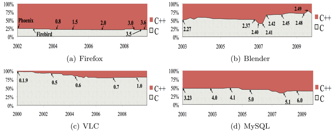
Figure 4.3: eLOC distribution per language.
