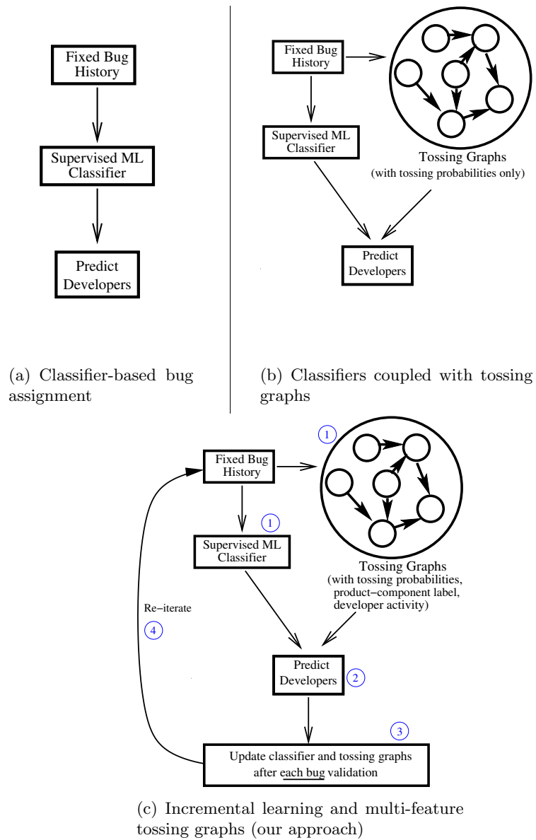
Figure 3.7: Comparison of bug assignment techniques.
