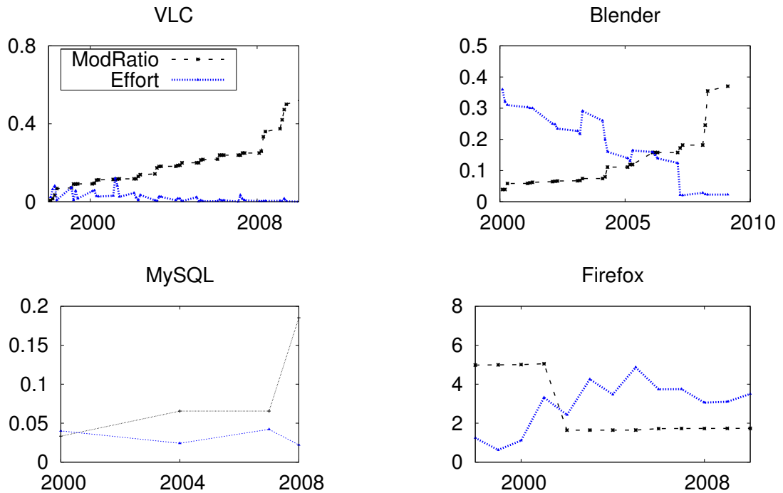
Figure 5.10: Change in ModularityRatio with change in Effort ; x -axis represents time.
