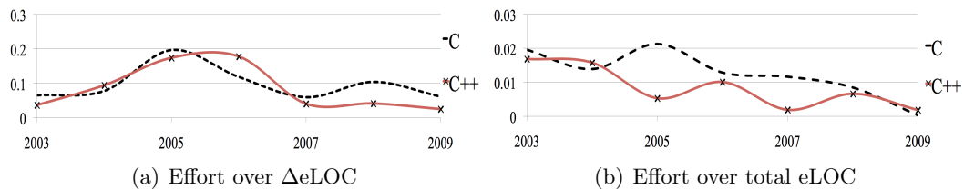
Figure 4.8: Maintenance Effort for Blender.
