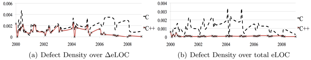
Figure 4.6: Defect Density in VLC.
