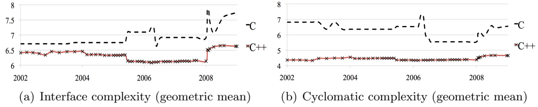
Figure 4.4: Internal Quality in Firefox.
