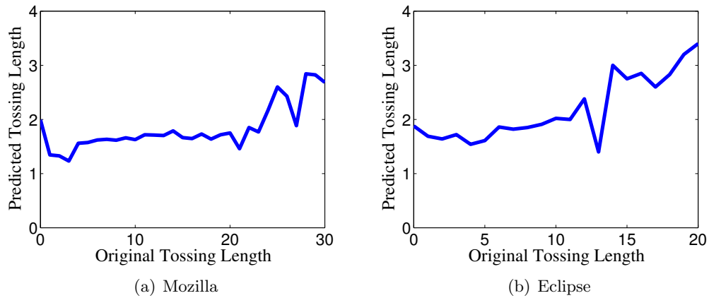
Figure 3.9: Average reduction in tossing lengths for correctly predicted bugs when using ML + Tossing Graphs (using both classifiers).
