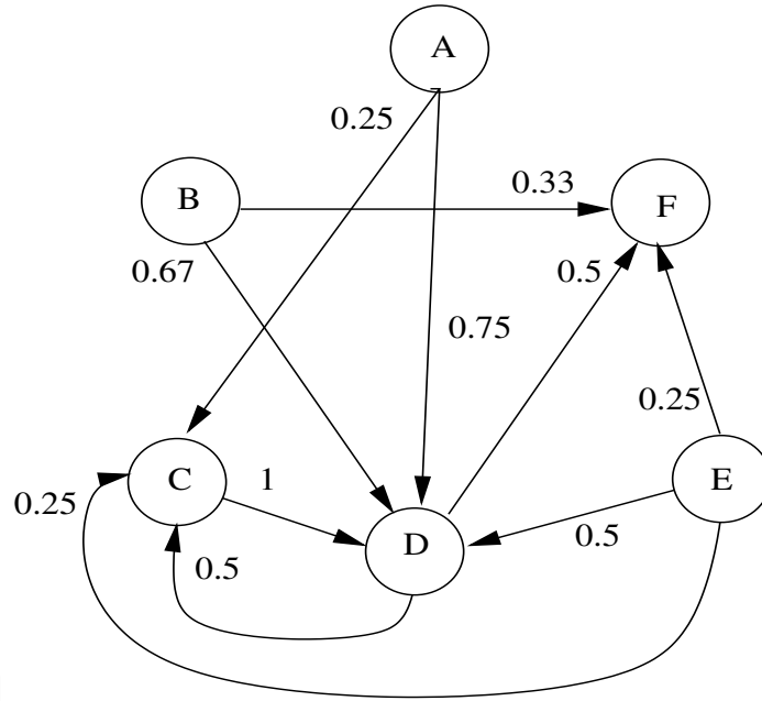
Figure 2.10: Tossing graph built using tossing paths in Table 3.1.
