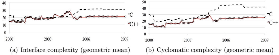
Figure 4.5: Internal Quality in VLC.
