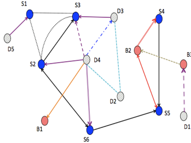
(b) Graph \mathbb{G}_{InterRepoDep} generated using relationships in Table 2.7(a)
