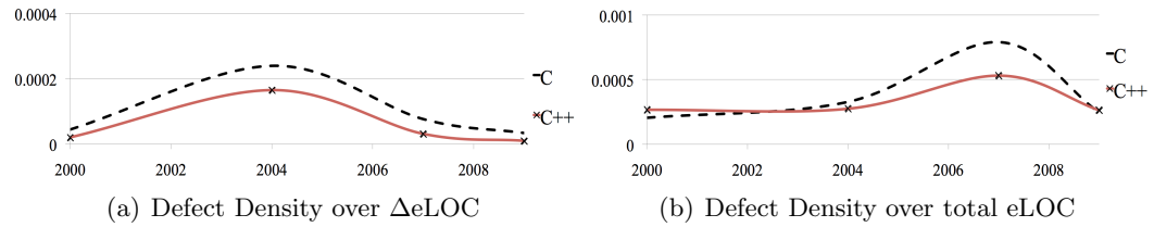
Figure 4.7: Defect Density in MySQL.
