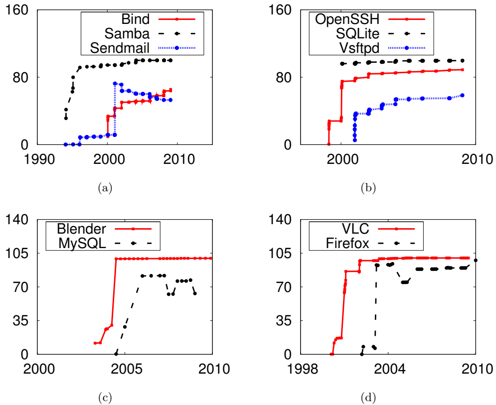
Figure 5.7: Change in Edit Distance over time.
