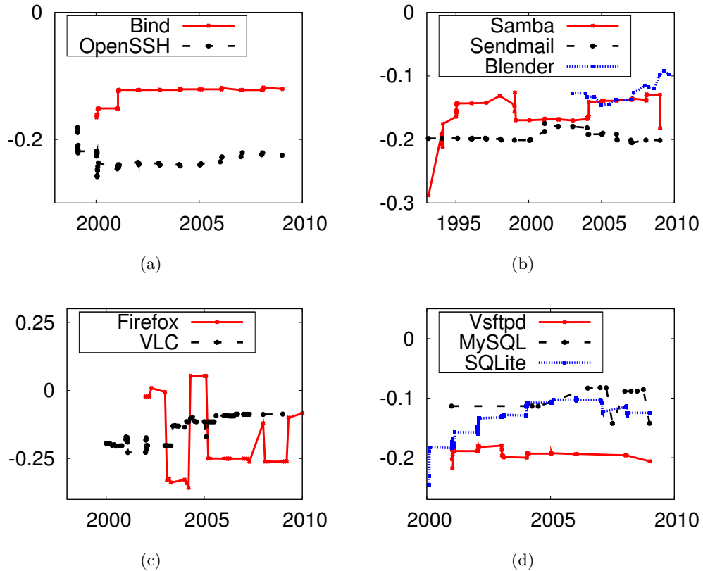
Figure 5.6: Change in Assortativity over time.
