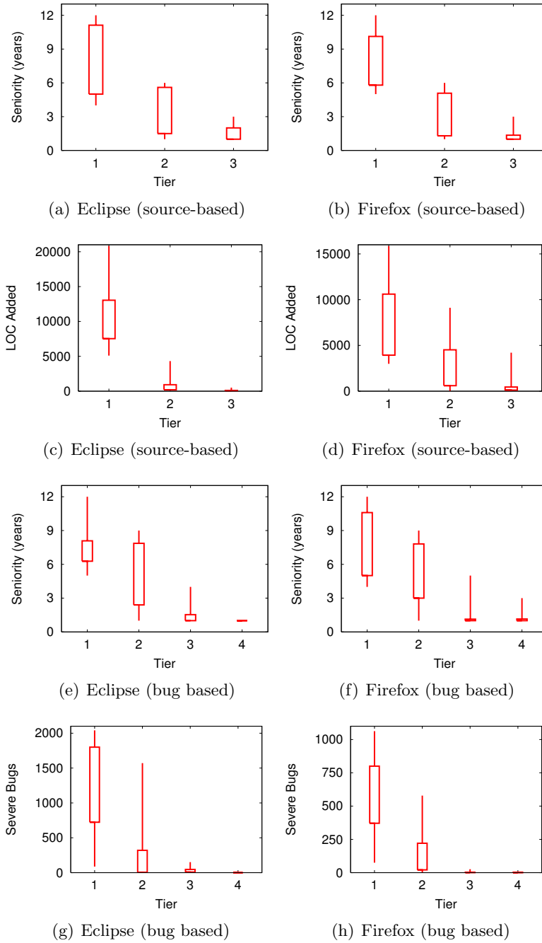
Figure 6.7: Tier distribution range per expertise metric.
