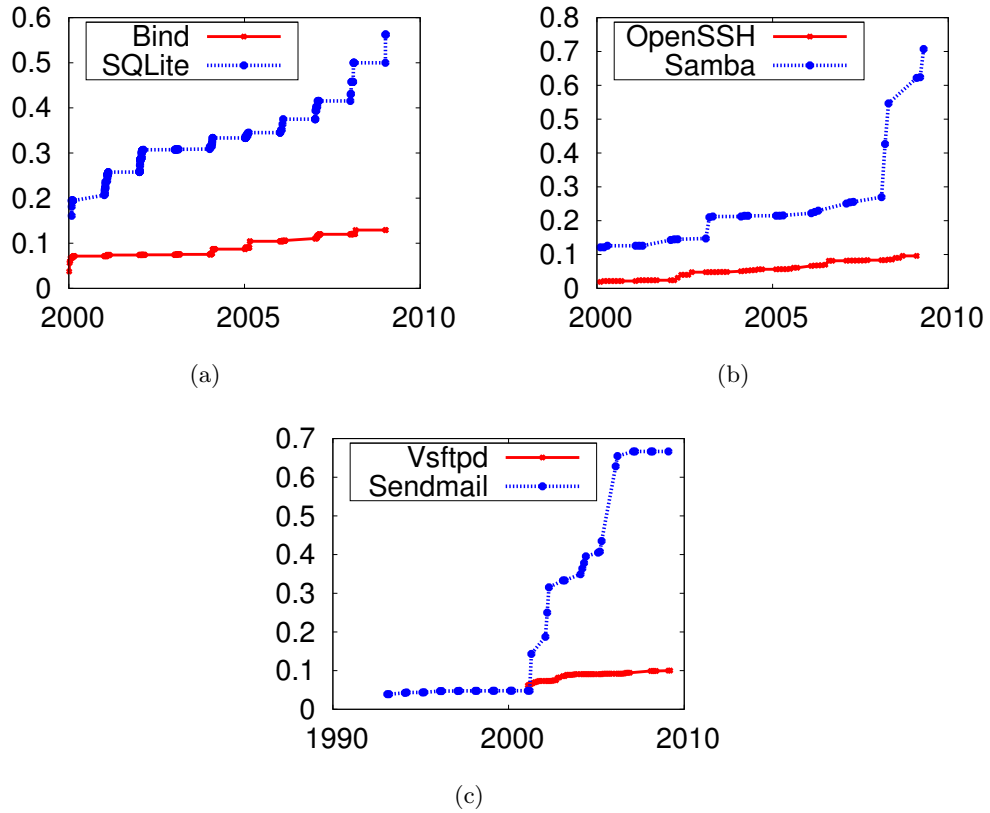
Figure 5.8: Change in Modularity Ratio over time.
