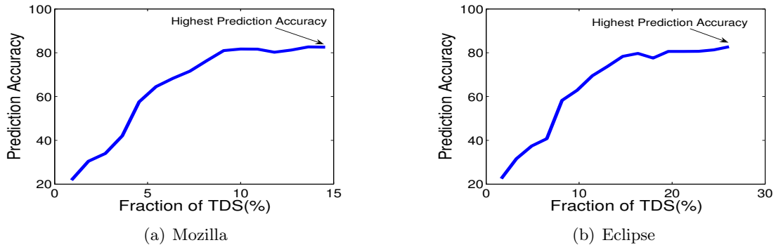
Figure 3.11: Change in prediction accuracy when using subsets of bug reports using Naïve Bayes classifier.
