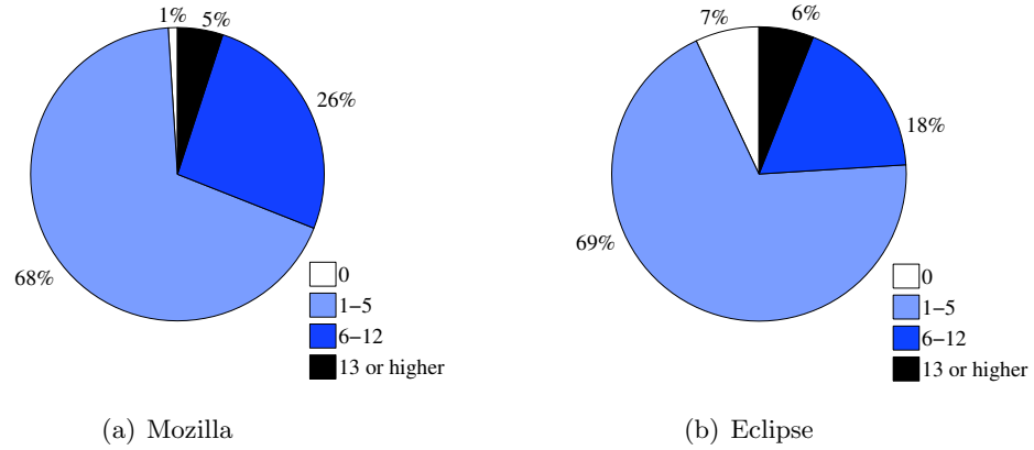
Figure 3.8: Original tossing length distribution for “fixed” bugs.
