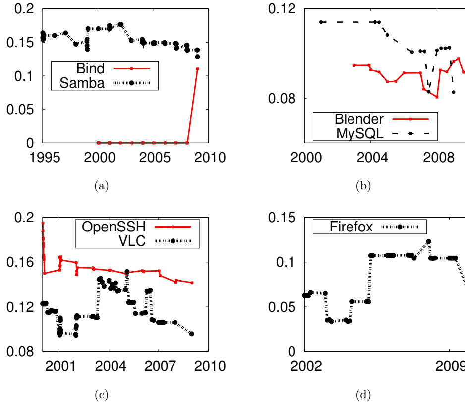
Figure 5.3: Change in Clustering Coefficient over time.
