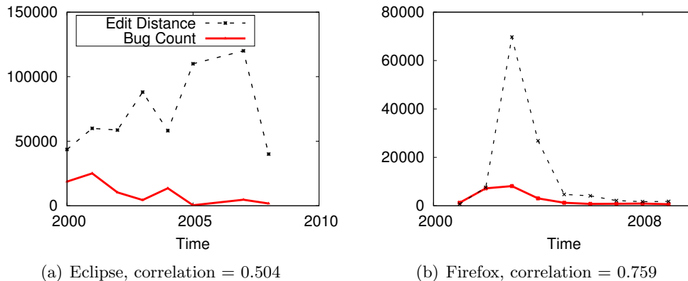
Figure 5.11: Change in collaboration graph Edit Distance v. Defect Count .
