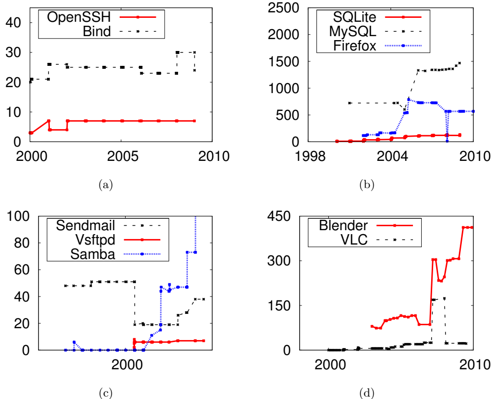
Figure 5.4: Change in Number of Cycles over time.
