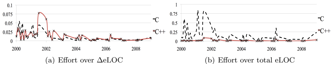
Figure 4.9: Maintenance Effort for VLC.
