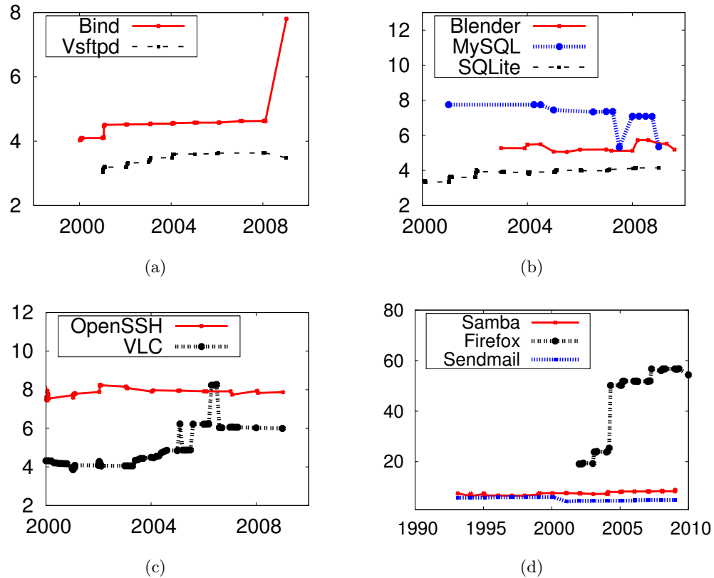
Figure 5.2: Change in Average Degree over time.
