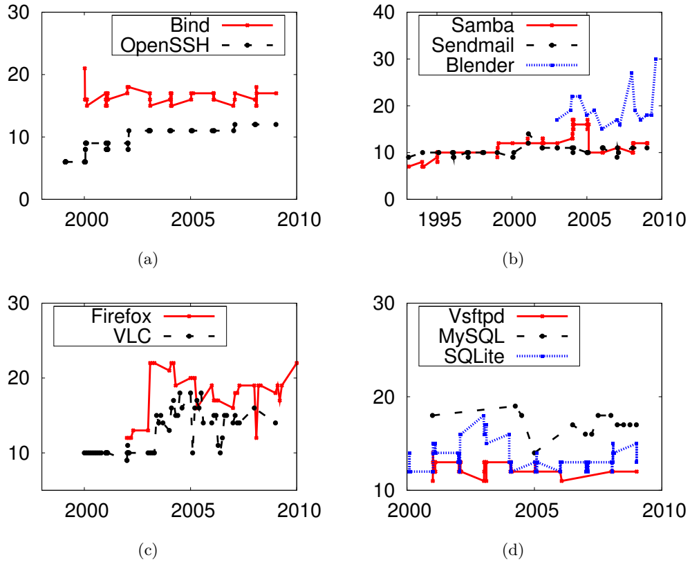
Figure 5.5: Change in Graph Diameter over time.
