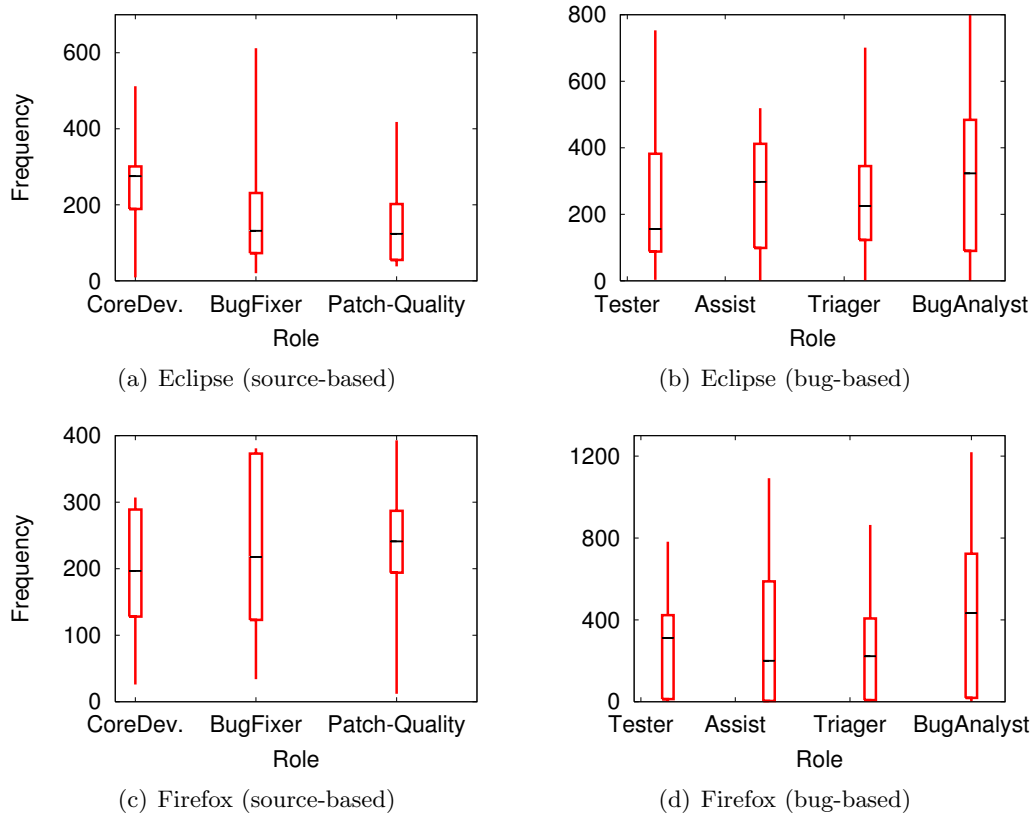
Figure 6.5: Frequency of contribution for each role.
