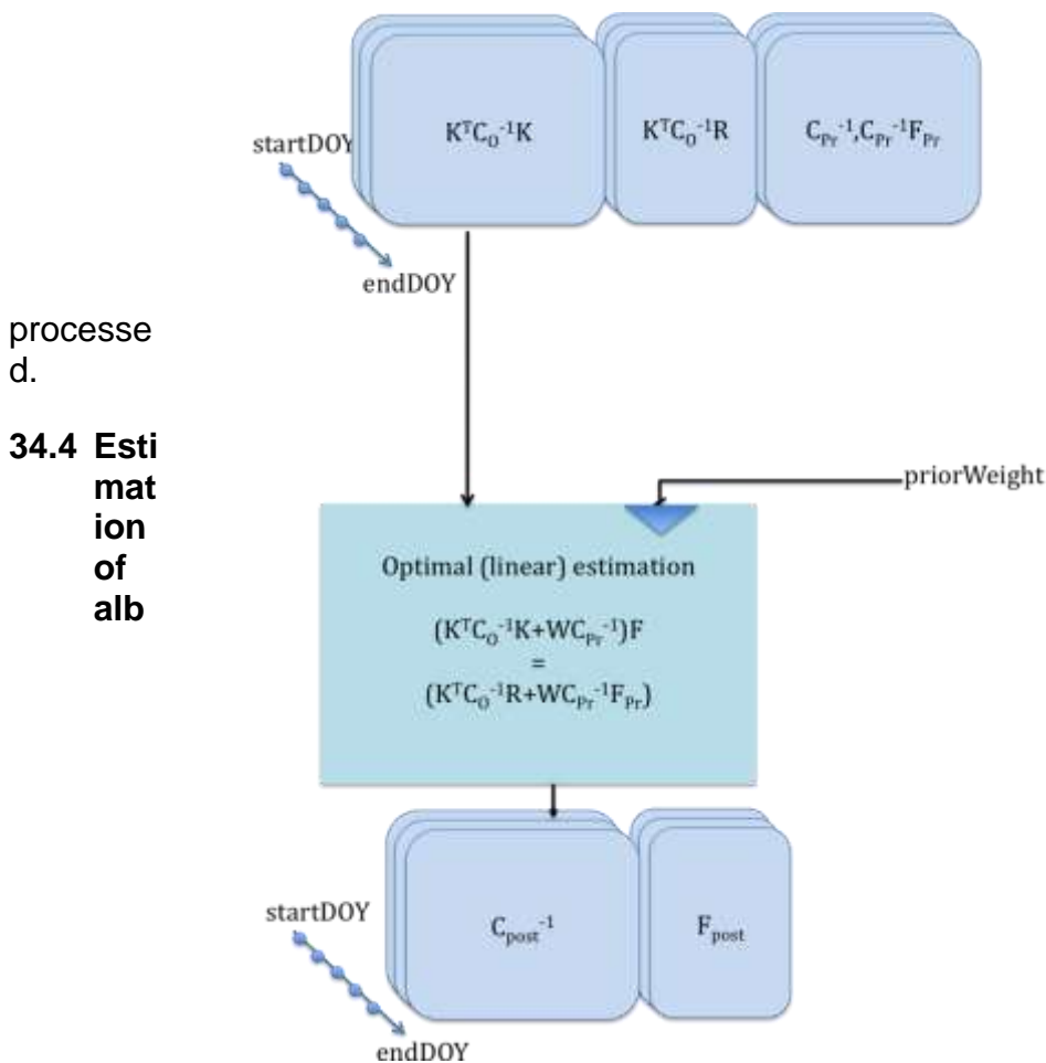
Figure 34-3. Optimal Estimator Flow diagram
