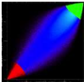
Figure 32-13. Tile h25v06: A) FCC mean f_0 (NIR,SW,VIS: RGB), DOY 001; B) in red strong negative correlation, in green strong positive correlation of VIS parameter f_0 and NIR parameter f_0 from smoothness parameter 0.5 and 1.0; C) correlation coefficients of VIS parameter f_0 in the x-axis and NIR parameter f_0 in the y-axis from smoothness parameter 0.5 and 1.0
