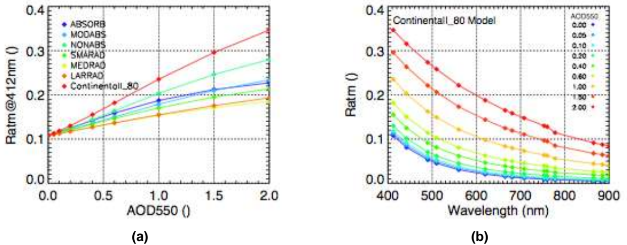
Figure 19-2: R_{atm,\lambda} as a function of the aerosol model. R_{atm,\lambda} in the MERIS band at 412nm is plotted as a function of AOD_{550} and the seven aerosol models in (a), while spectral R_{atm,\lambda} for the continental model is represented in (b). The reference input configuration is VZA=30^\circ , SZA=30^\circ , RAA=120^\circ , ELEV=200m .
