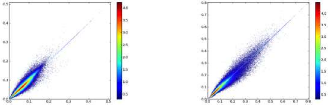
Figure 32-5. On the left, mean f_0 h18v04 DoY 001 1.0 vs 0.5, on the right, mean f_0 h18v04 DoY 145 1.0 vs 0.5
