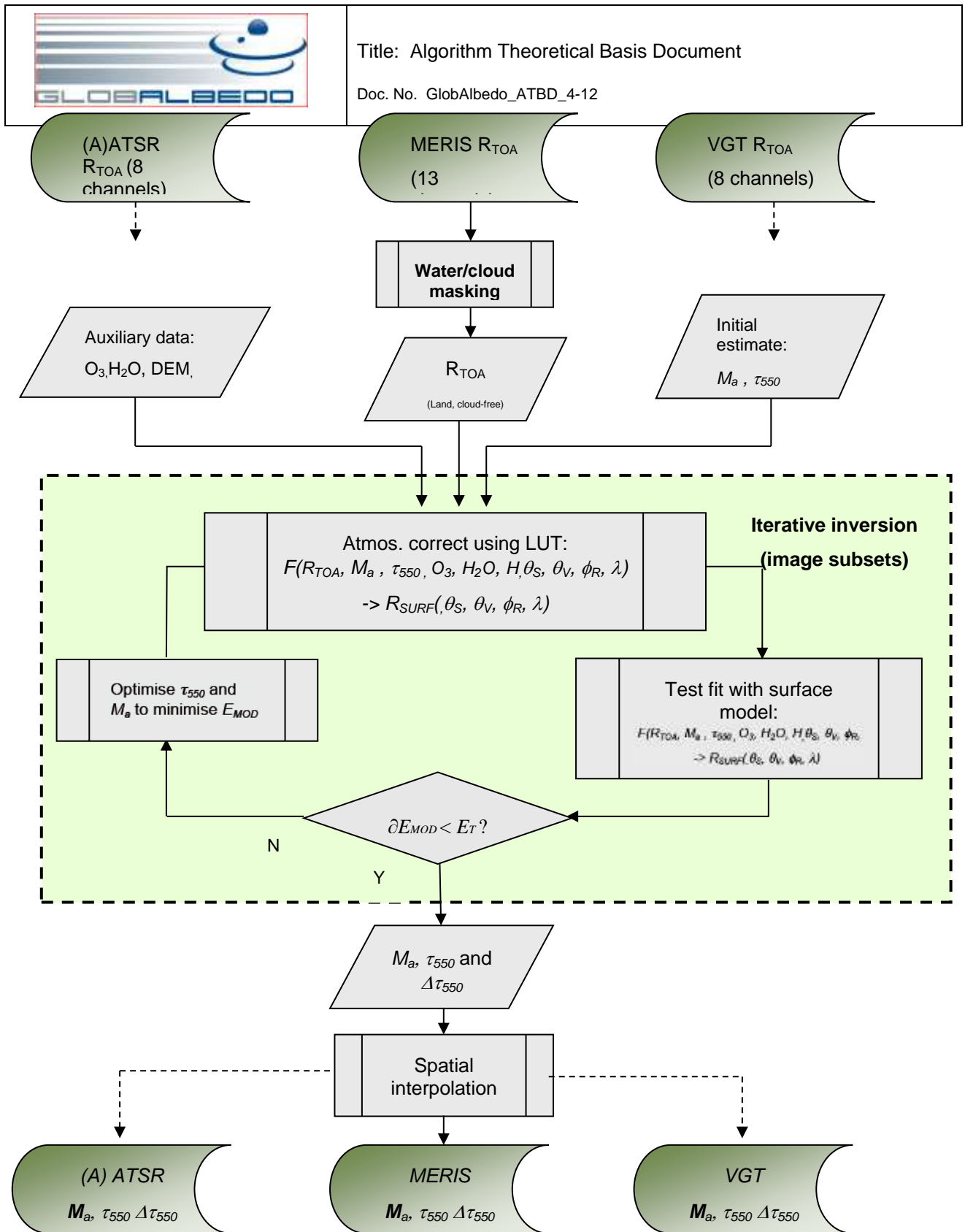
Figure 19-1: Outline processing algorithm for retrieval of aerosol properties for GlobAlbedo
