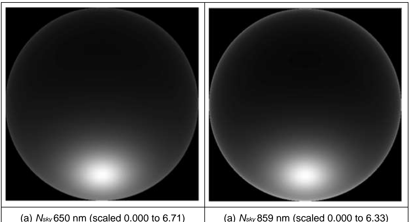
Figure 31-1. Polar plot of normalised sky radiance for a solar zenith angle of 45°.
