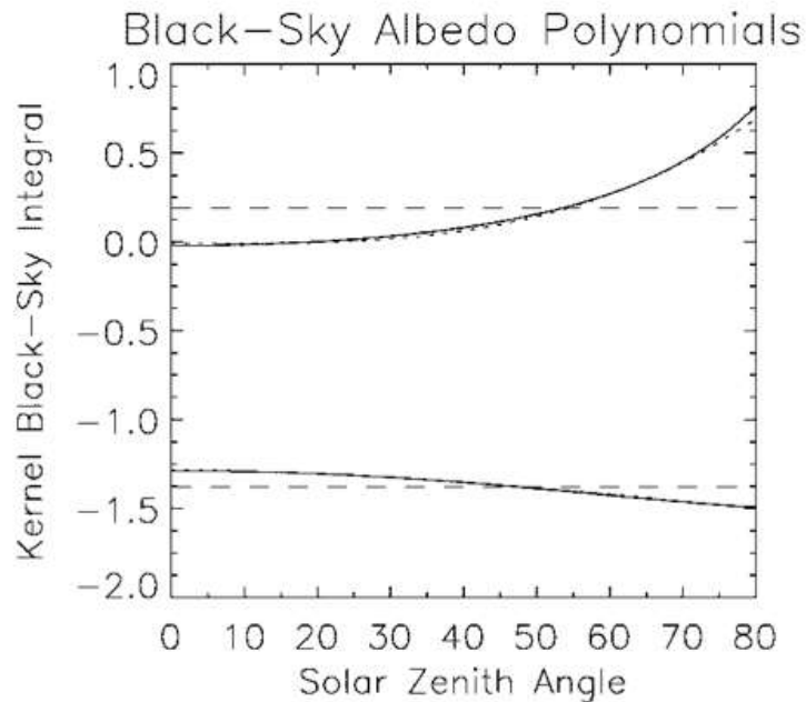
Figure 31-8. (From Lucht et al., 2000) Polynomial representation of black sky albedo as a function of solar zenith angle. Values shown for RossThick and of the LiSparse-R kernel (solid lines) and their polynomial representations (dotted lines).
