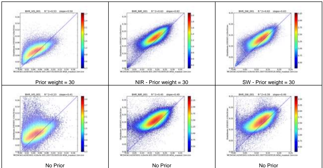
Figure 34-6. BHR inter-comparison of GlobAlbedo, with and without the use of the Prior and MCD43A3, for tile h18v04 DoY = 1
