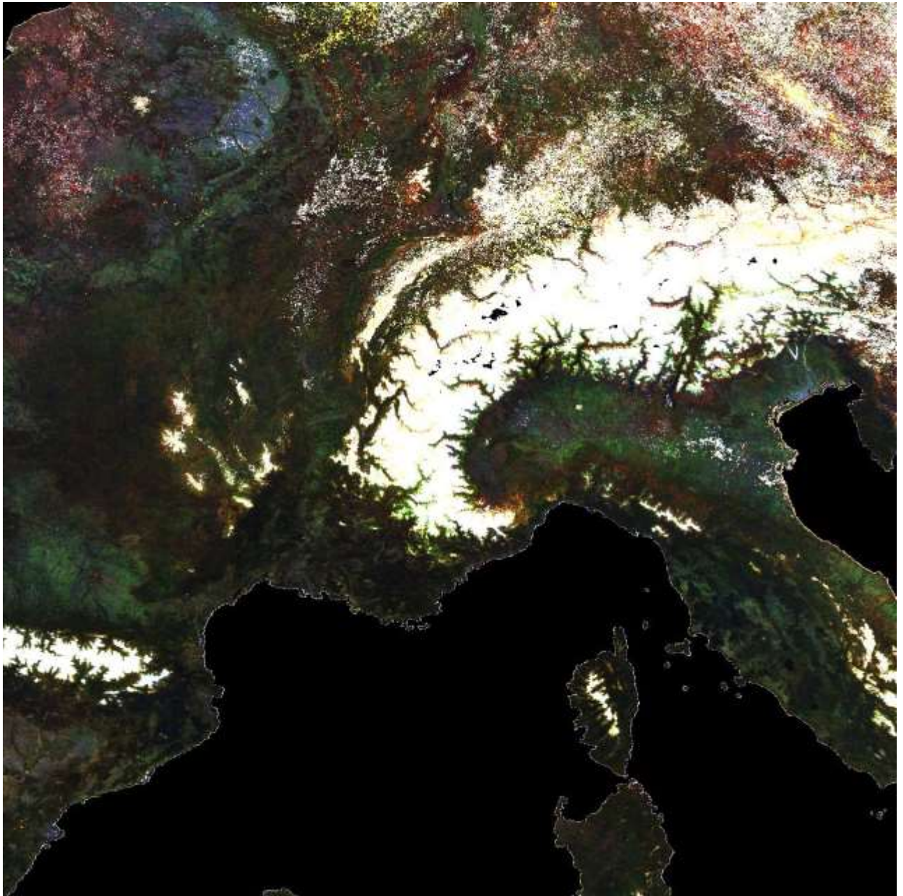
Figure 32-20. MODIS climatology VIS 'snow free' uncertainty in bihemispherical reflectance (white sky albedo) for (DOY 009, 041, 105 on RGB) scaled [0.000:0.065]
