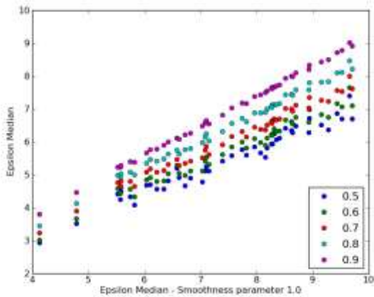
Figure 32-15. Temporal profile of epsilon A: peak of histogram, B: median and C: scatter plot of epsilon median for different smoothness parameters; Tile h18v04, with correlation information
