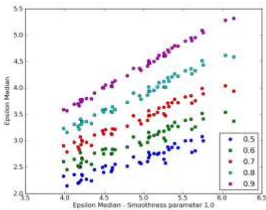
Figure 32-16. Temporal profile of epsilon A: peak of histogram, B: median and C: scatterplot of epsilon median from smoothness parameter 1.0 and 0.5 to 0.9; Tile h18v04, without correlation information
