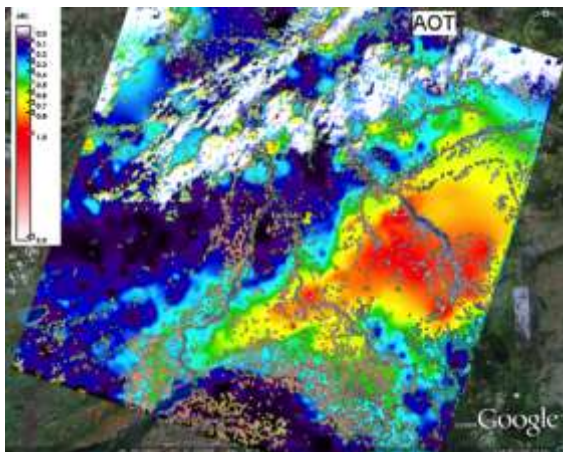
Figure 20-1: a) RGB composite (1600n, 870n, 550f) around Tomsk Aeronet station on 15. May 2005. b) AOT retrieval for AATSR with angular approach only c) AOT uncertainty.
