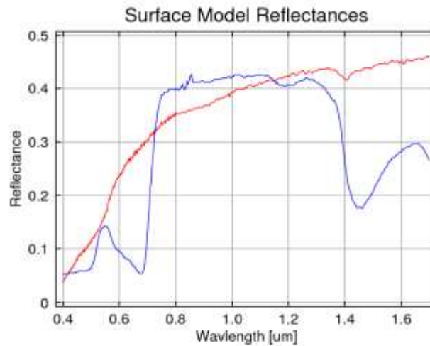
Figure 19-3: Surface reflectance model spectra for soil and vegetation
