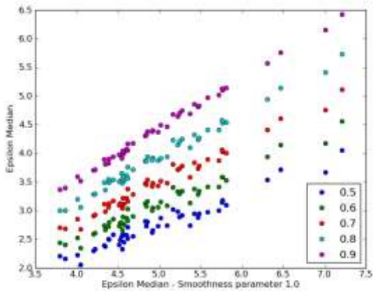
Figure 32-18. Temporal profile of epsilon A: peak of histogram, B: median and C: scatter plot of epsilon median from smoothness parameter 1.0 and 0.5 to 0.9; Tile h25v06, epsilon statistics without correlation information
