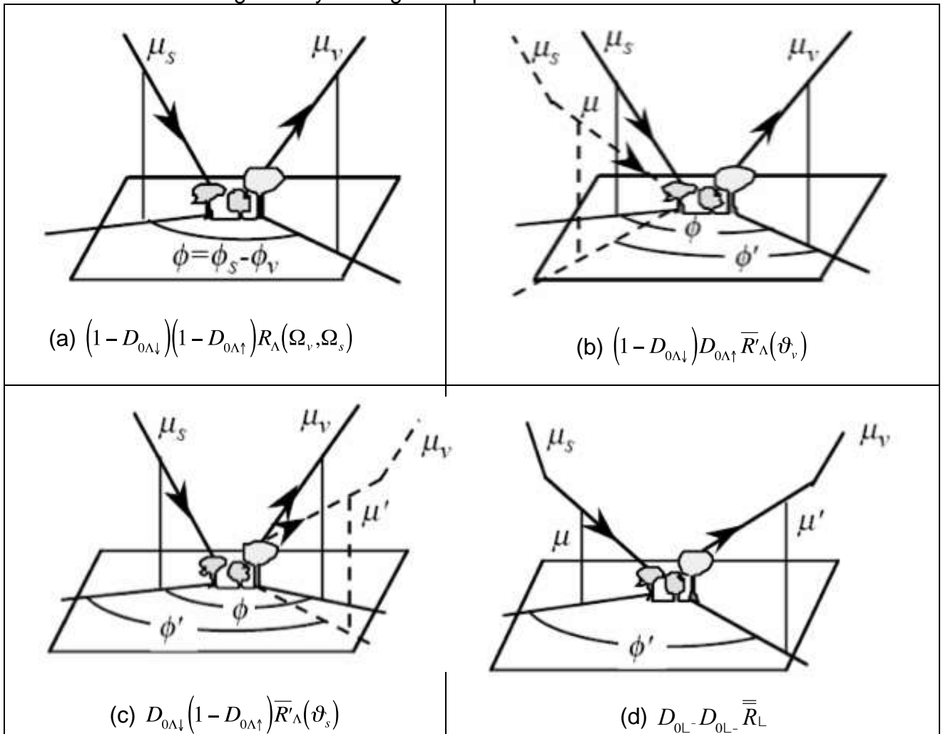
Figure 31-2. Atmospheric interaction mechanisms (from Vermote et al. 2006 6 )
