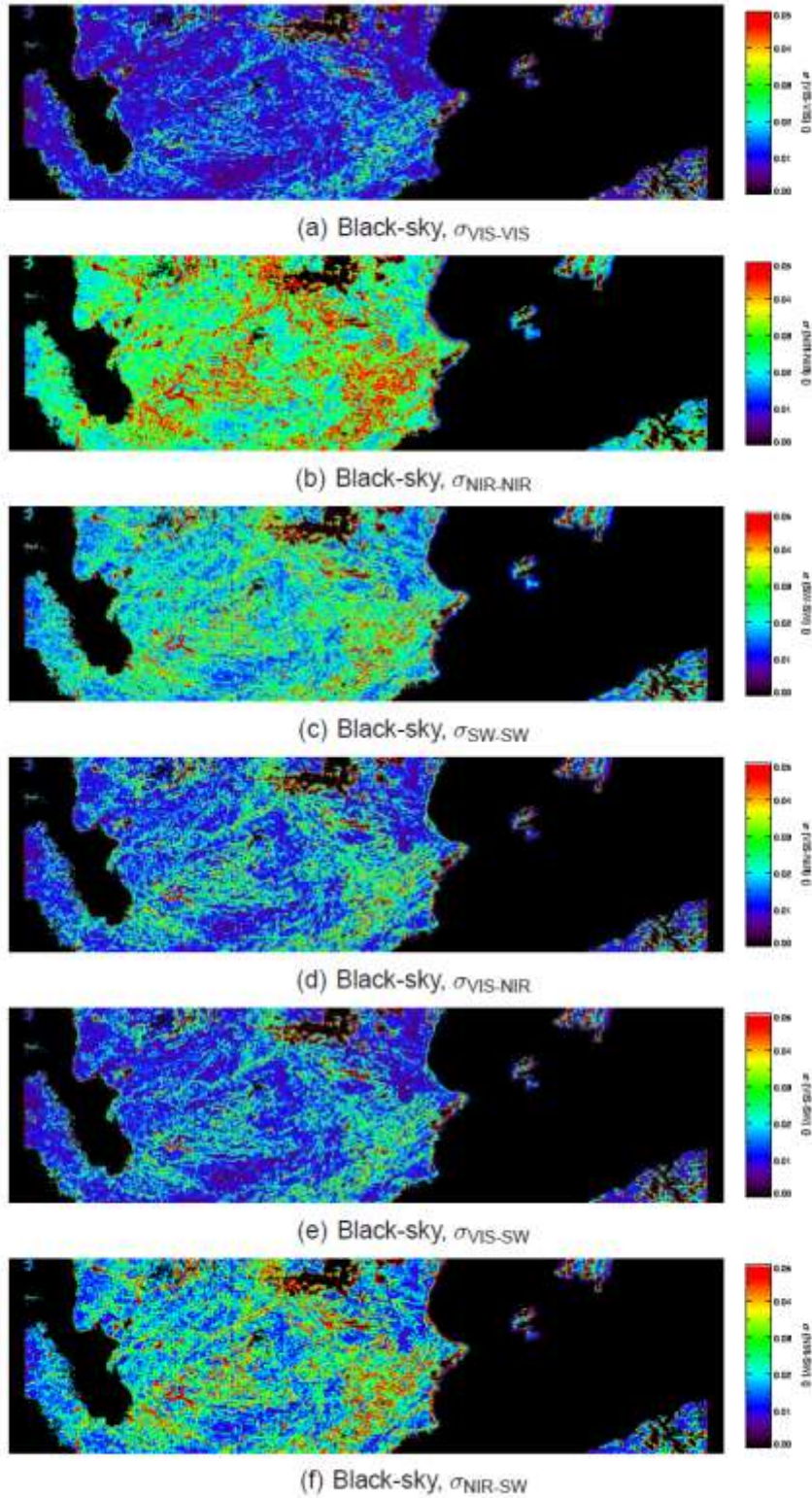
Figure 22: \sigma_{\Lambda} derived from a MERIS Level-1b image acquired over the Iberian Peninsula on 14/7/2003.
