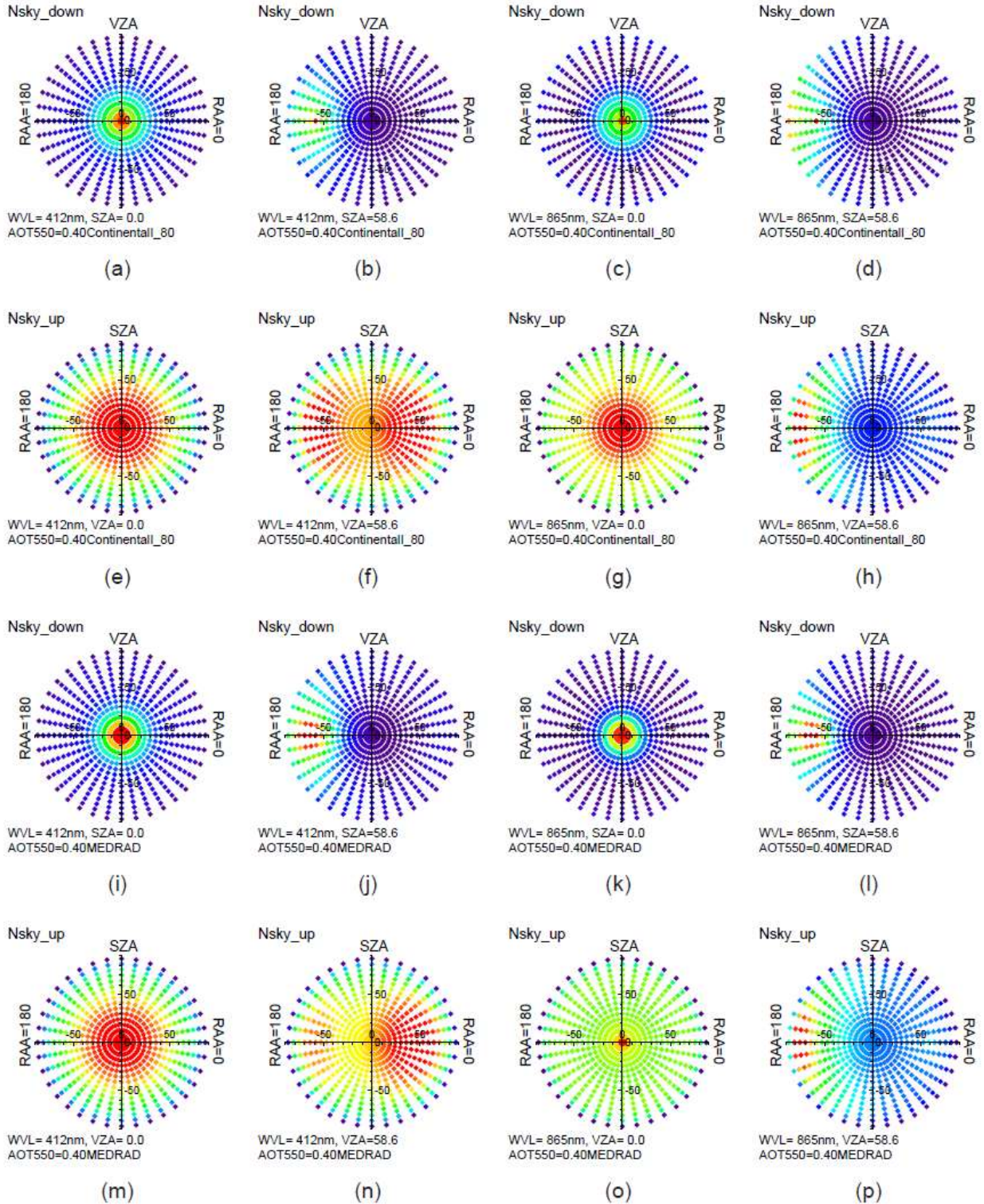
Figure 13: Sample N_{\text{sky}\downarrow}(\Omega_s) and N_{\text{sky}\uparrow}(\Omega_v) functions for AOD550=0.4 and different reference SZA and VZA, aerosol models and spectral wavelengths. Colours indicate the intensity of scattering for each direction in the hemisphere (purple is minimum intensity, red is maximum).
