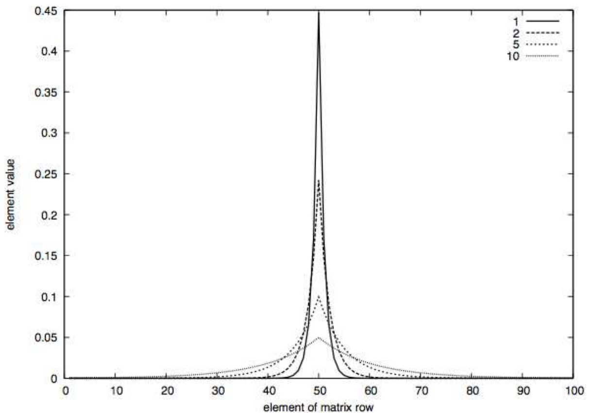
Figure 31-14. From Quaife (2009): Inverse differential operator for varying values of \gamma
