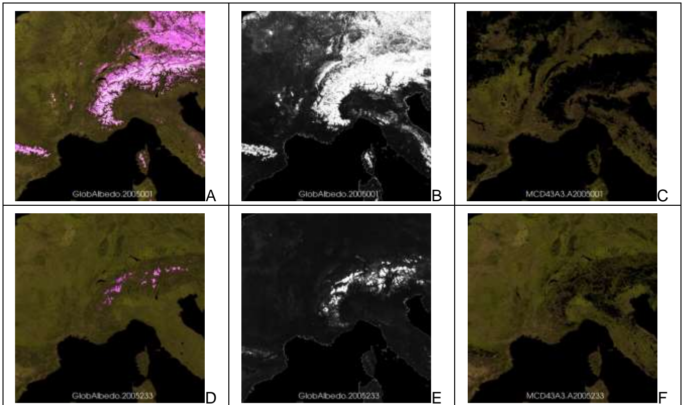
Figure 34-5. Upper row shows products for DoY 1, bottom row for DoY 233 for tile h18v04. Panels A and D show a false colour composite of GlobAlbedo BHR SW,NIR,VIS (RGB), panels B and E the BHR uncertainty in the SW scaled 0:0.1,
