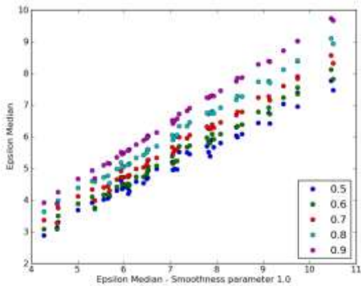
Figure 32-17. Temporal profile of epsilon A: peak of histogram, B: median and C: scatterplot of epsilon median from smoothness parameter 1.0 and 0.5 to 0.9; Tile h25v06, epsilon statistics with correlation information
