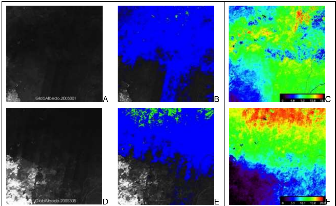
Figure 35-3. Top row shows products for DoY 1, bottom row for DoY 305 for tile h19v08. Panels A and D depict BHR uncertainty in the SW scaled 0:0.1, panels B and E the SW relative error, areas in green have 0-5% error, in blue 5-10% error, panels C and F show the weighted number of samples.
