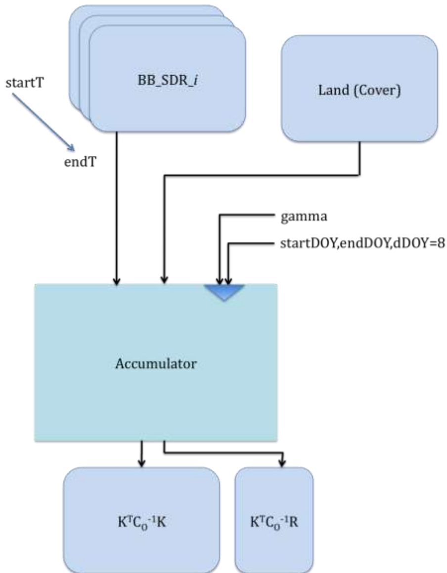
Figure 34-2. Accumulator Flow diagram
