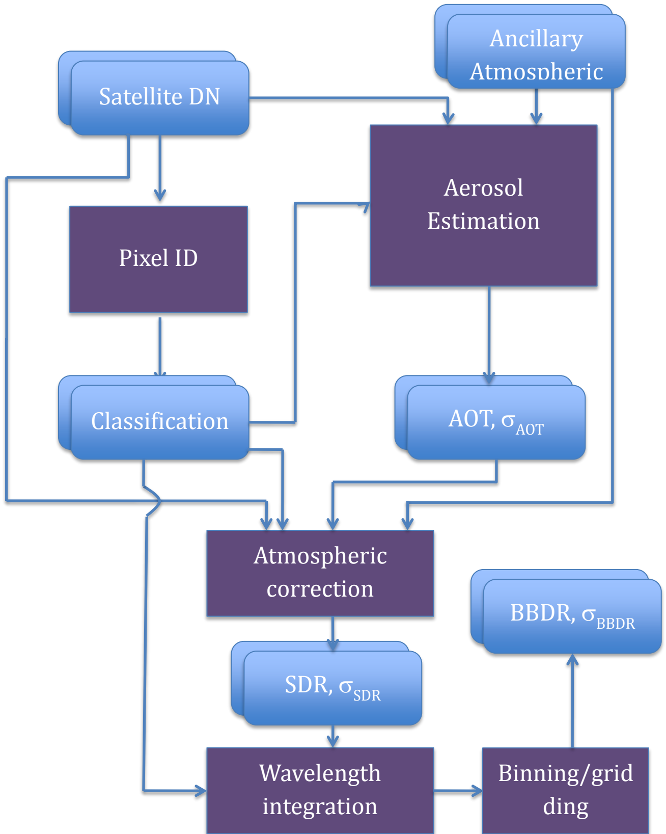
Figure 3-3. GlobAlbedo Pre-processing Steps
