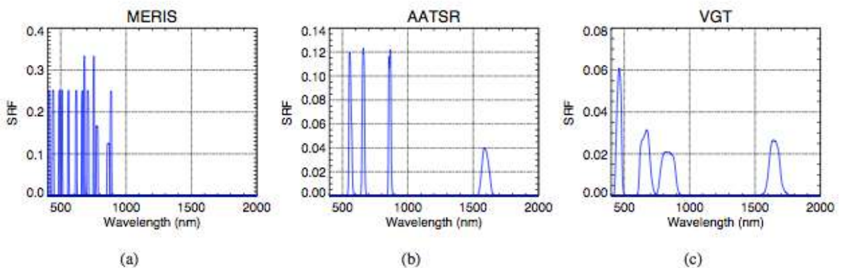
Figure 3-1. Spectral response functions of the different sensors (from GlobAlbedo_BBDR_ATBD_V2.0, 2010)
