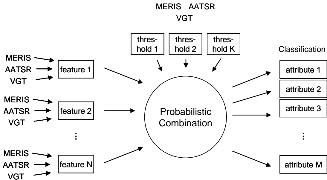
Figure 11-3: Unified Pixel Classification Scheme
