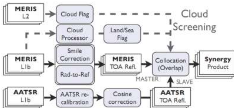
Figure 11-2: Flowchart of the MERIS and AATSR synergy preprocessing module
