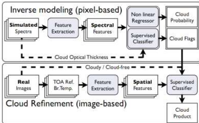
Figure 11-1: Overview of synergistic cloud classification algorithm
