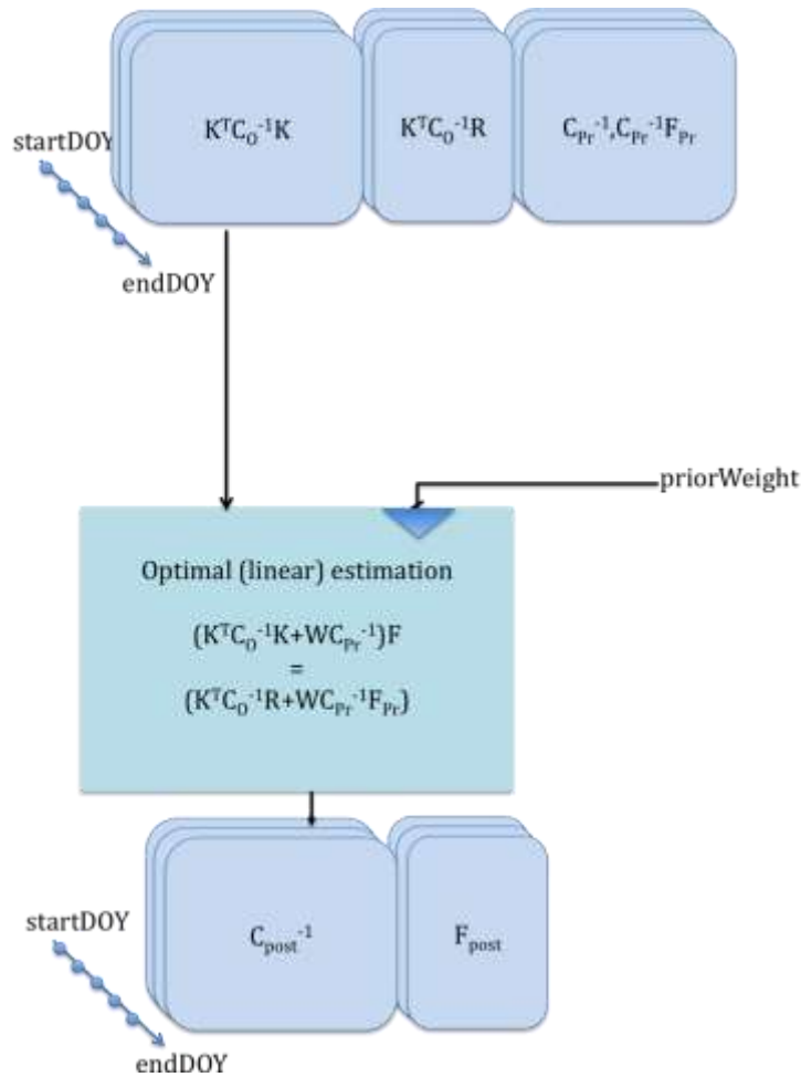
Figure 34-4. Albedo Estimator Flow diagram
