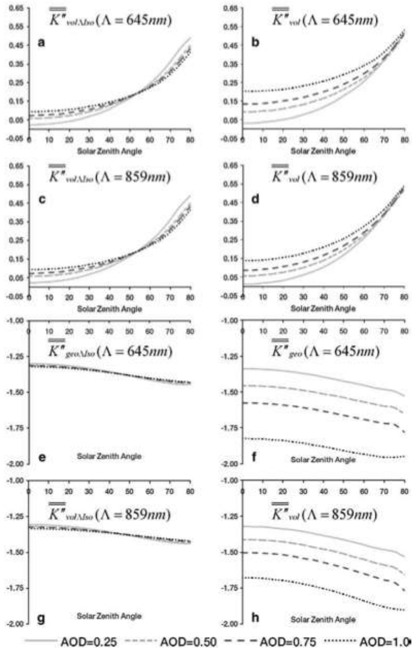
Figure 31-7. Angular integrals of kernels for varying aerosol optical depth (AOD) and solar zenith angles for MODIS red and NIR bands. The left column shows terms K''_{x,\Lambda}(\vartheta_s) assuming isotropic illumination for the diffuse component. The results in the right column are for N_{sky} -weighting of the terms. From Roman et al. (2010).
