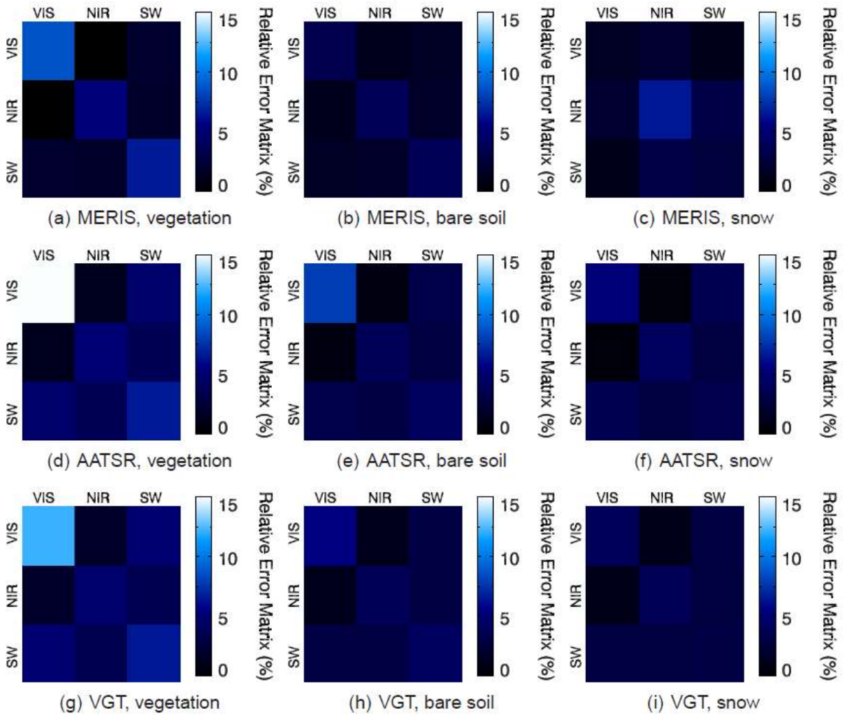
Figure 19: Same as Fig. 18 for the relative error matrix \sigma_{\Lambda}^{rel} defined in Eq. 5.18.
