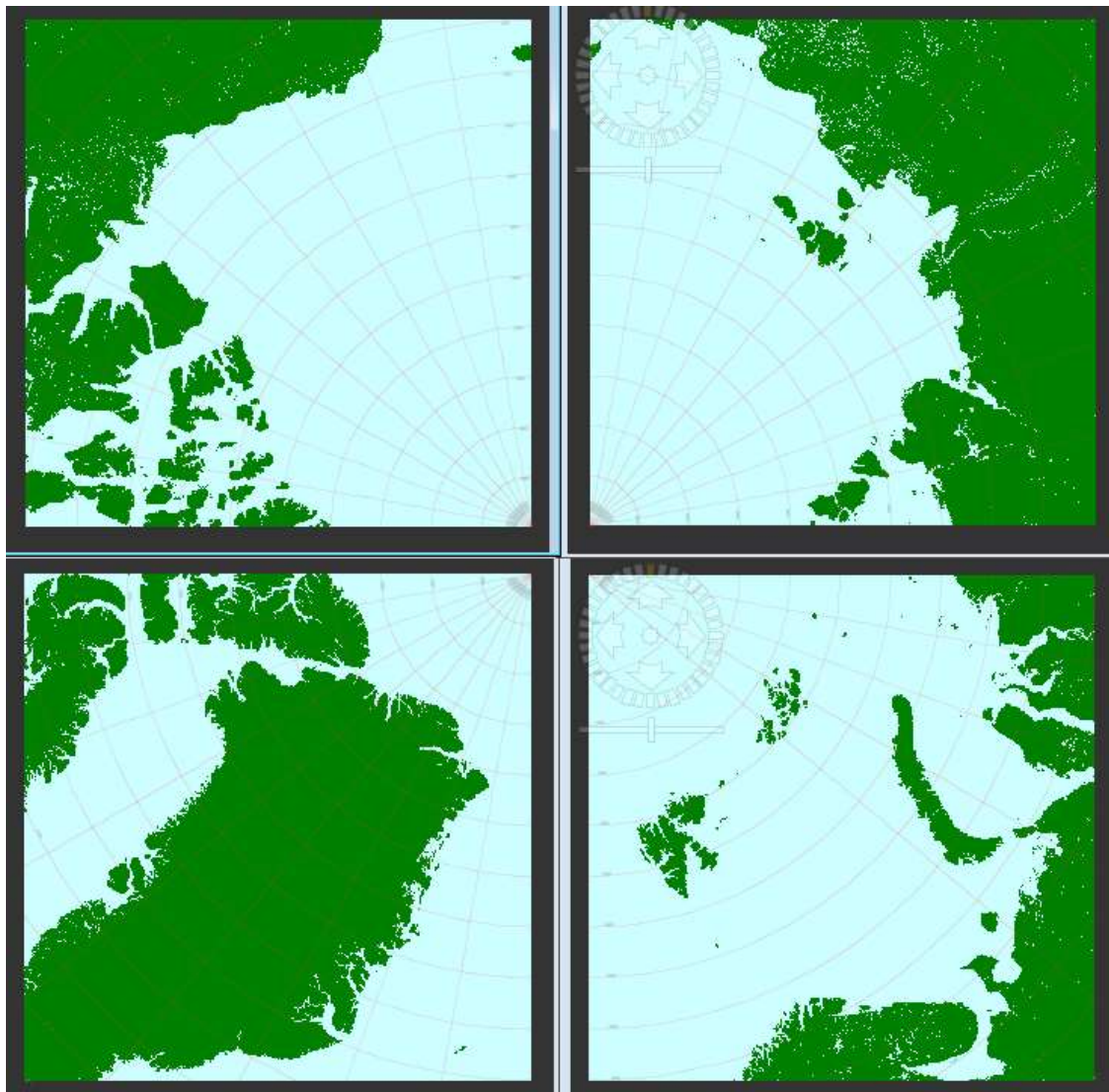
Figure 34-1. Polar 'quadrant tiles' used in GlobAlbedo sea-ice albedo computation.
