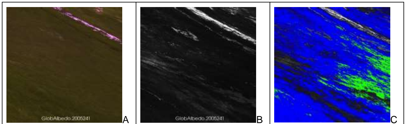
Figure 35-2. Panels A shows a false colour composite of GlobAlbedo BHR SW,NIR,VIS (RGB), panel B uncertainty in the SW scaled 0:0.1, panel C the SW relative error, areas in green have 0-5% error, in blue 5-10% error. Products are for DoY=241 tile h22v02
