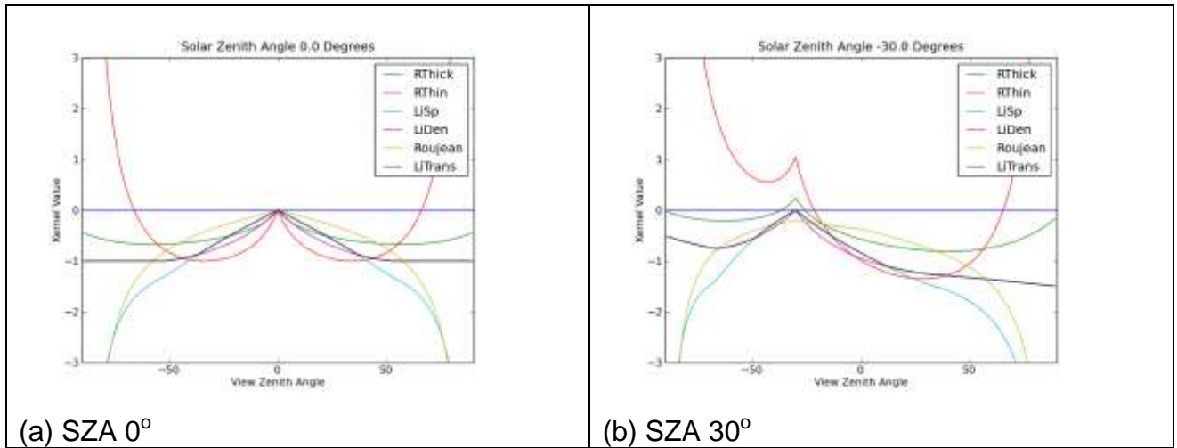
Figure 31-5. Linear Kernels (Principal plane) -- non-reciprocal Li and Ross HS
