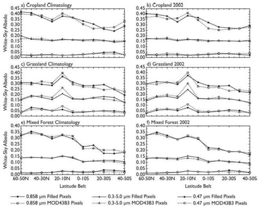
FIG. 8. Mean diffuse bihemispherical (white sky) albedo values computed by 10° latitude belts for three bands (0.47- and 0.86-μm narrowband and the 0.3-5.0-μm shortwave broadband) during the 16-day period of 12-27 Jul (data-day 193). Trends are computed for three ecosystem classes: (a), (b) cropland, (c), (d) grassland, and (e), (f) mixed forest from (left) the 5-yr aggregate climatology and (right) the 2002 single-year albedo data.
