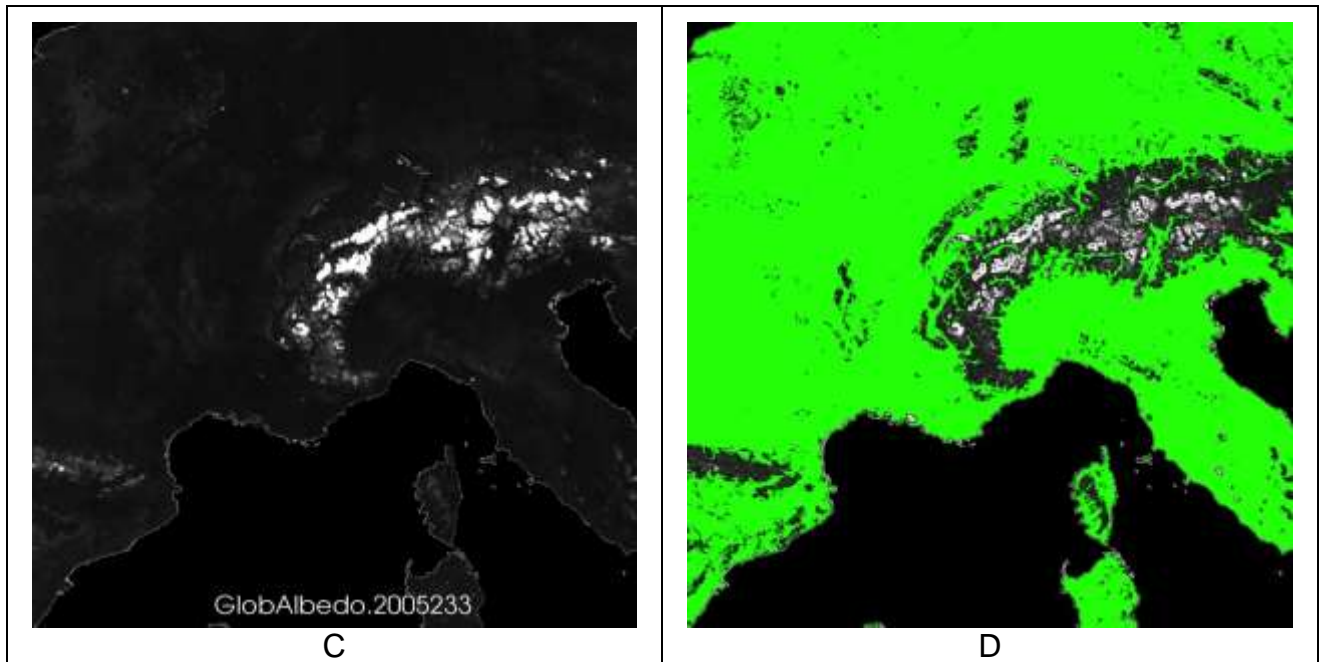
Figure 35-1. Top row shows products for DoY 1, bottom row for DoY 233 for tile h18v04. Panels A and C depict BHR uncertainty in the SW scaled 0:0.1, panels B and D the SW relative error, areas in green have 0-10% error.
