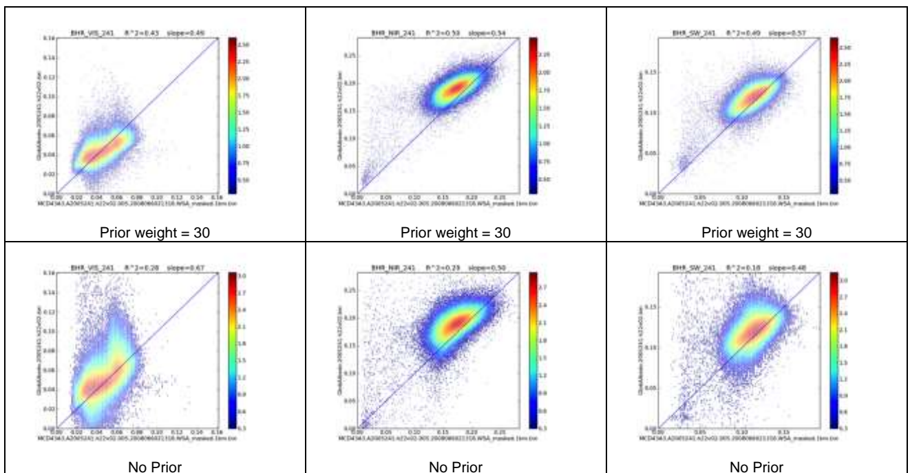
Figure 34-9. BHR inter-comparison of GlobAlbedo, with and without the use of the Prior and MCD43A3, for tile h22v02 DoY = 241
