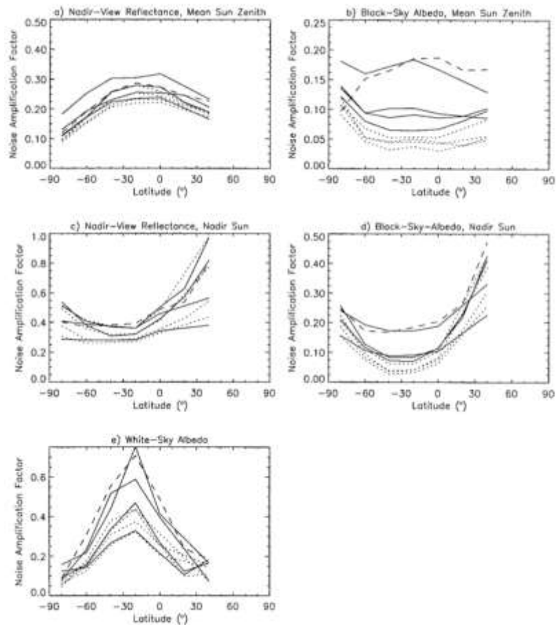
Figure 31-11. From Lucht and Lewis (2000). Noise sensitivity of the modified RPV BRDF model.
