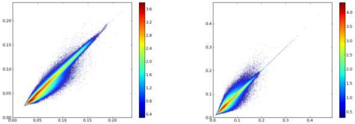
Figure 32-6. On the left, mean f_0 h19v08 DoY 001 1.0 vs 0.5, on the right, mean f_0 h19v08 DOY 145 1.0 vs 0.5
