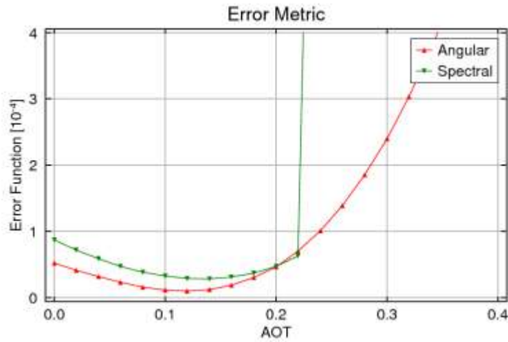
Figure 19-4: Example of variation of angular and spectral error metrics with AOT for a vegetated scene (Tomsk) for AATSR and MERIS respectively.
