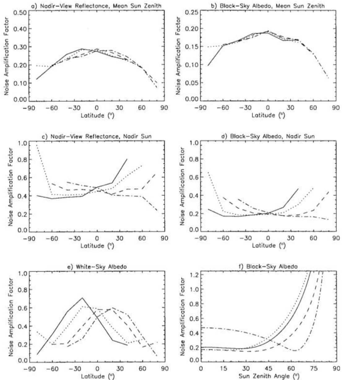
Figure 31-9. From Lucht and Lewis (2000). Noise sensitivity of the RossThick-LiSparse BRDF model. Weights of determination (noise amplification factors) are shown as a function of latitude for different 16-day time periods throughout the first half of the year, the time progressing through solid, dotted, dashed and dashed-dotted curves (days of year 0, 48, 96 and 144). Panel (f) shows the noise sensitivity of black-sky albedo extrapolation as a function of sun zenith angle for sample latitudes -60^{\circ} , -40^{\circ} , 0^{\circ} and 40^{\circ} latitude (solid, dotted, dashed, dashed-dotted curves), for sampling during the first 16-day period of the year. The terms 'mean sun zenith' and 'nadir sun' refer to evaluations at the mean sun zenith angle at which the observations were made at each respective latitude and for the case of a solar zenith angle extrapolated to nadir.
