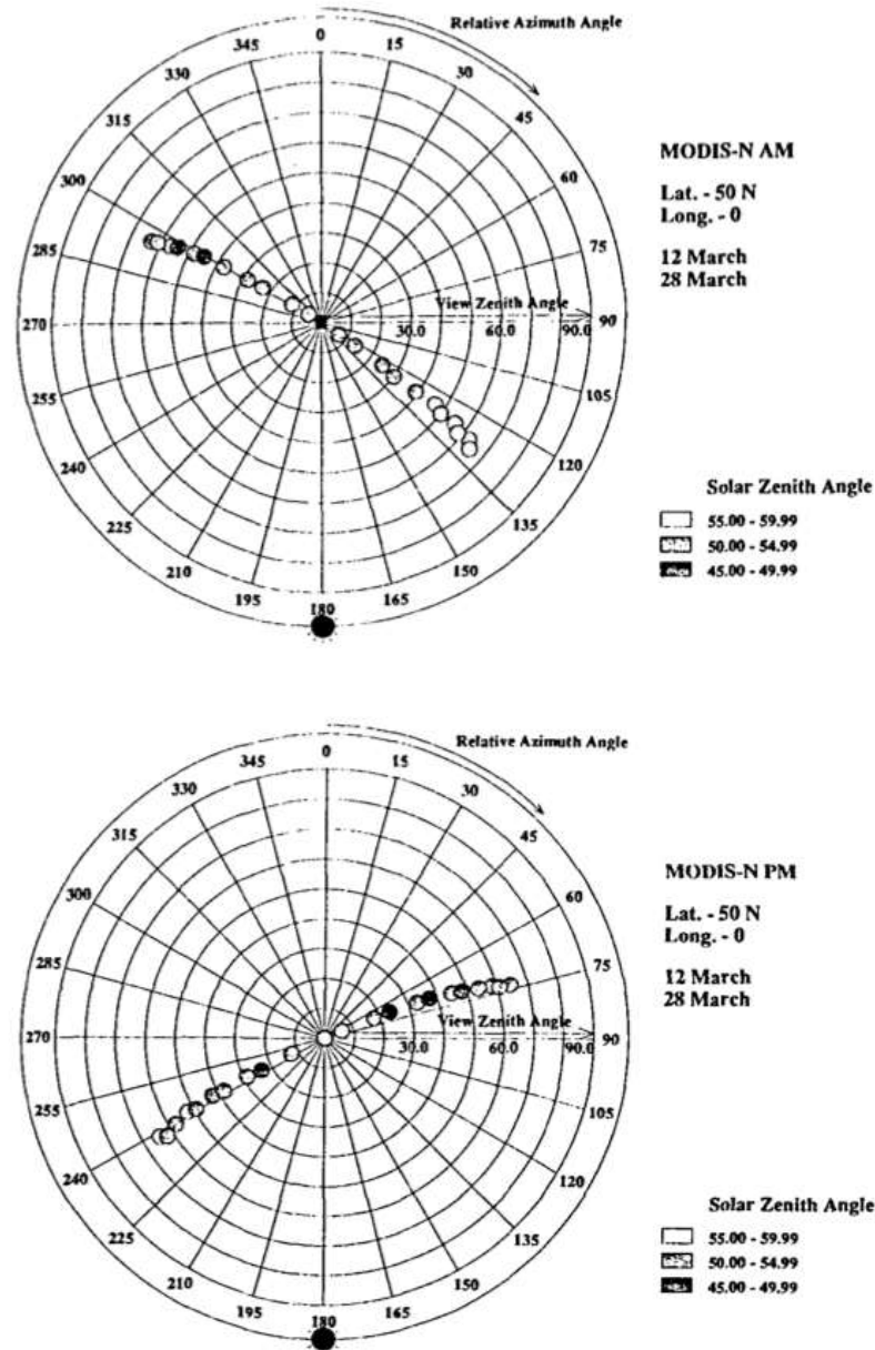
Figure 31-12. From Barnsley et al. 1994. Angular sampling of MODIS instruments (labelled MODIS-N) for the two platforms (Terra and Aqua). Concentric rings denote 10° increments of view zenith angle, ranging from 0° (i.e. nadir) at the center of the plot to 90° at the edge. Radial lines denote 15° increments of view azimuth angle,
