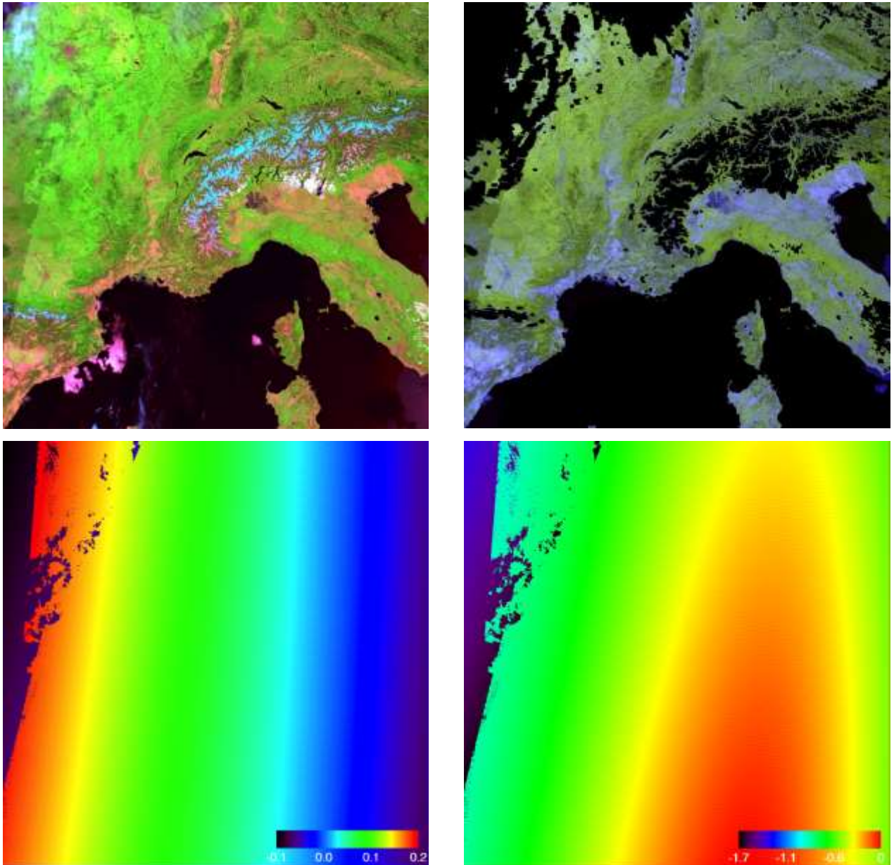
Figure 37-1. On the upper left corner, daily surface reflectance product derived from MODIS in a false color composite bands 7,2,1 RGB, on the upper right corner the conversion to broadband masked from clouds and snow, the Ross-Thick kernel is shown on the lower right corner and, the Li-Sparse reciprocal kernel on the bottom right.
