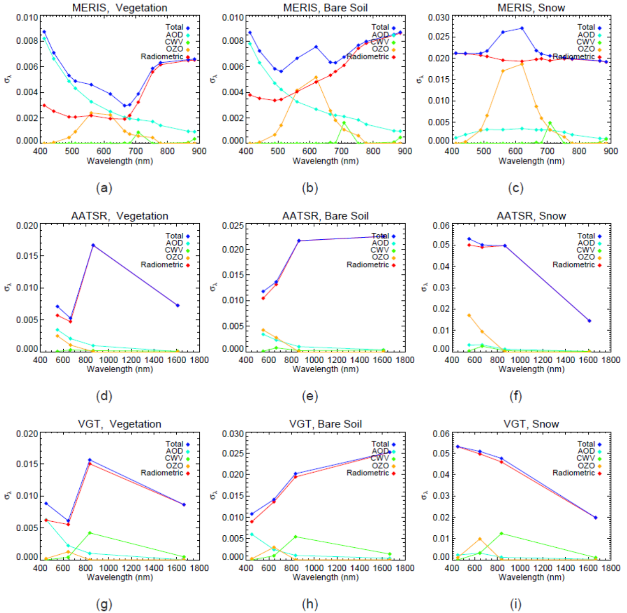
Figure 17: SDR retrieval error ( \sigma_\lambda ) associated to each of the error sources considered for the three instruments and three characteristic land cover types. The reference input configuration is VZA=15^\circ , SA=35^\circ , RAA=123^\circ , ELEV=450 m, AOD=0.25 , CWV=2 g cm^{-2} , OZO=0.265 atm cm^{-1} , \sigma_{AOD}^{rel}=30\% , \sigma_{CWV}^{rel}=20\% , \sigma_{OZO}^{rel}=30\% . Input reflectance patterns are those in Fig. 15.
