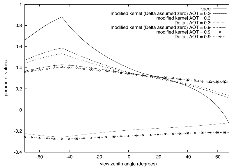
(b) Geometric kernel terms
