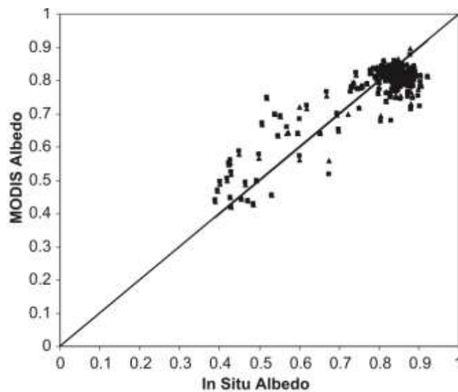
Figure 32-3. Comparison between clear-sky MODIS 16-day albedo and 16-day in situ albedo for both the Black sky albedo and white sky albedo, combined for all Greenland stations (from Stroeve et al., 2005).
