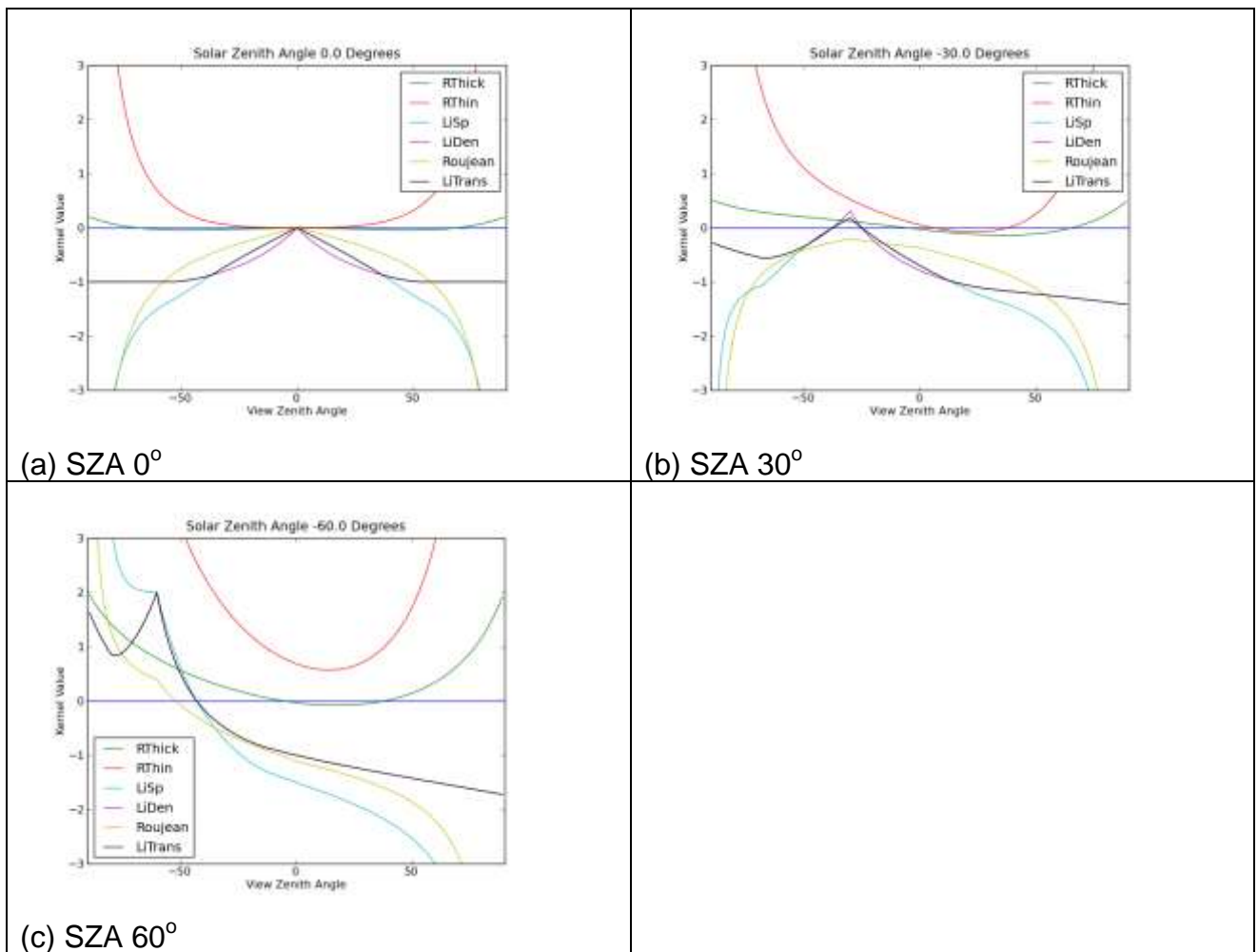
Figure 31-6. Linear Kernels (Principal plane) – Reciprocal Li
