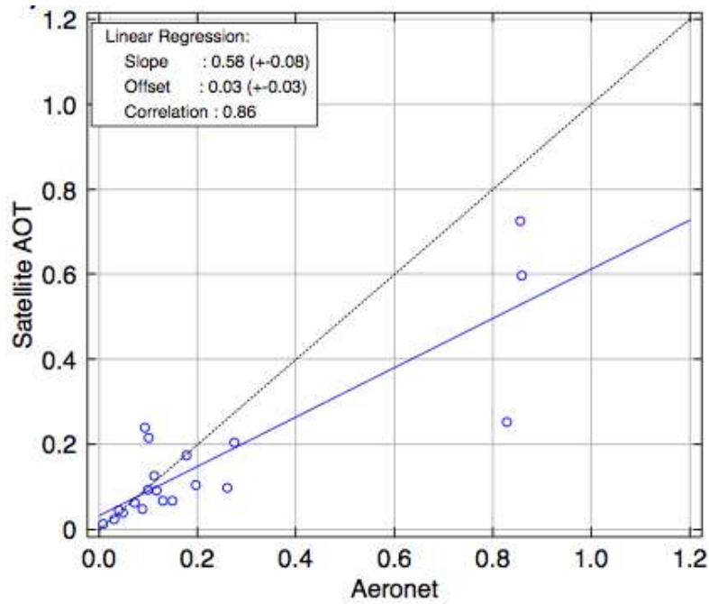
Figure 20-5: Results of AATSR retrieval compared with AERONET sites (DDV targets only).
