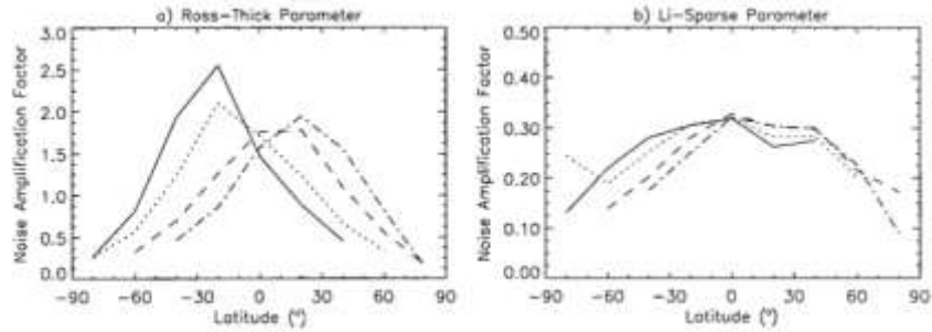
Figure 31-10. From Lucht and Lewis (2000). Impact of angular sampling on estimates of the linear model parameters. Lines have same meanings as in figure 12.
