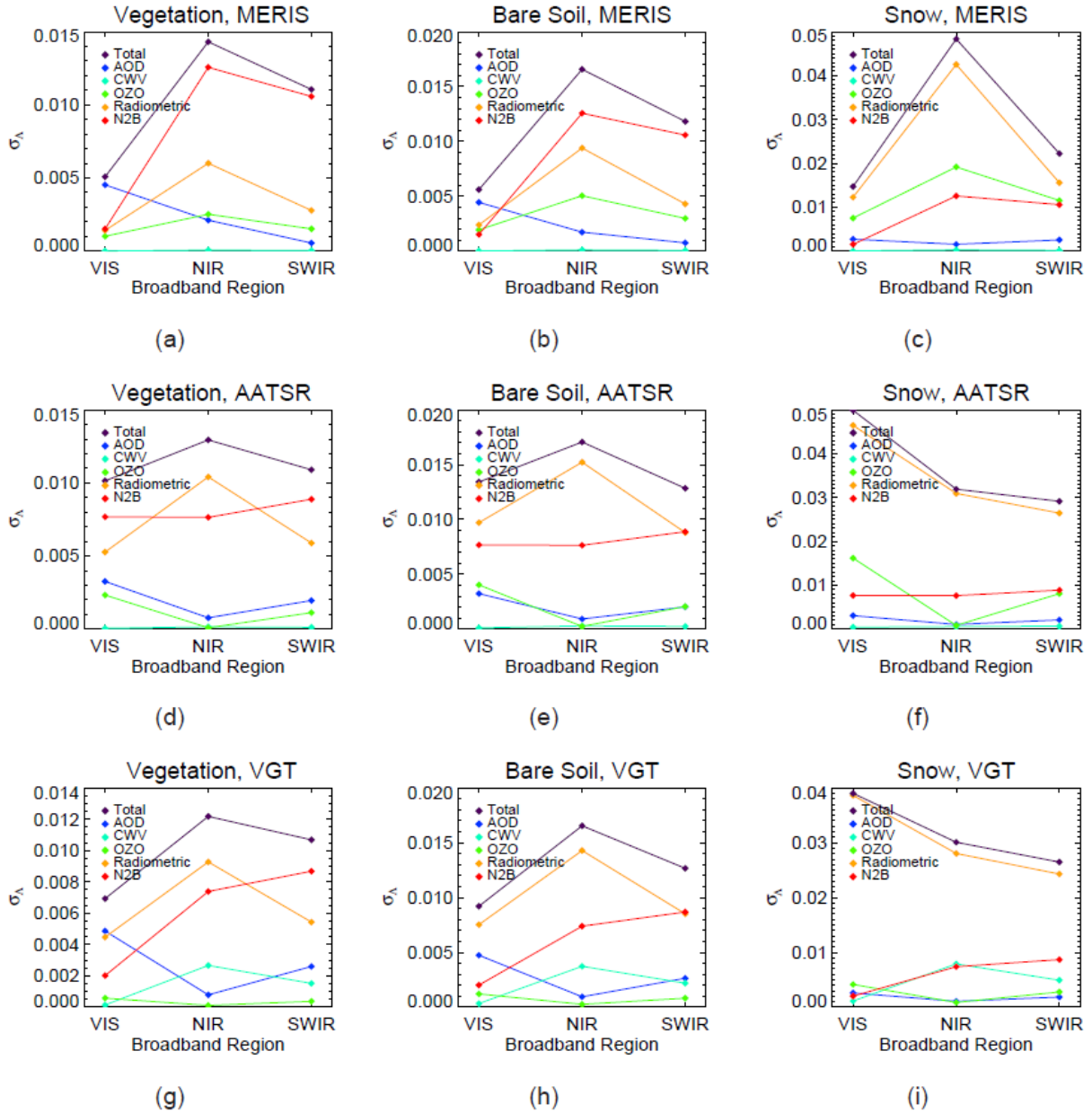
Figure 8: Contribution of the different error sources considered in this study to the diagonal terms of \sigma_{\Lambda} for the vegetation, soil and snow spectral patterns in Fig. 15 and the three instruments. The reference input configuration is VZA=15^{\circ} , SZA=35^{\circ} , RAA=123^{\circ} , ELEV=450 m, AOD=0.25 , CWV=2 g cm ^{-2} , OZO=0.265 atm cm ^{-1} , \sigma_{AOD}^{rel}=30\% , \sigma_{CWV}^{rel}=20\% , \sigma_{OZO}^{rel}=30\% .
