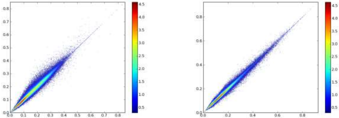
Figure 32-8. On the left, mean f_0 h25v06 DOY 001 1.0 vs 0.5, on the right, mean f_0 h25v06 DOY 145 1.0 vs 0.5
