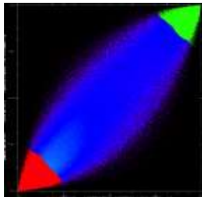
Figure 32-11. Tile h18v04: A) FCC mean f_0 (NIR,SW,VIS: RGB), DOY 001; B) in red strong negative correlation, in green strong positive correlation of VIS parameter f_0 and NIR parameter f_0 from smoothness parameter 0.5 and 1.0; C) correlation coefficients of VIS parameter f_0 in the x-axis and NIR parameter f_0 in the y-axis from smoothness parameter 0.5 and 1.0
