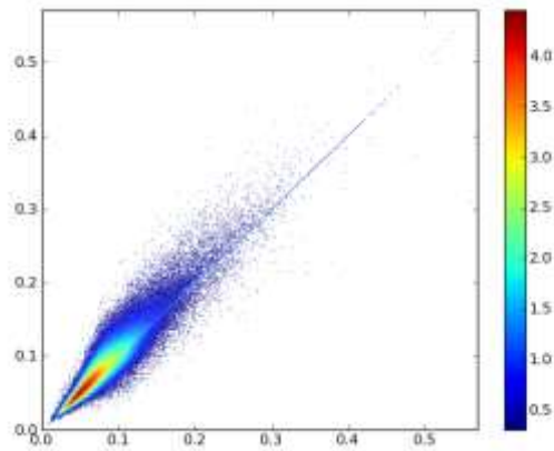
Figure 32-7. Mean f_0 h22v02 DOY 145 1.0 vs 0.5
