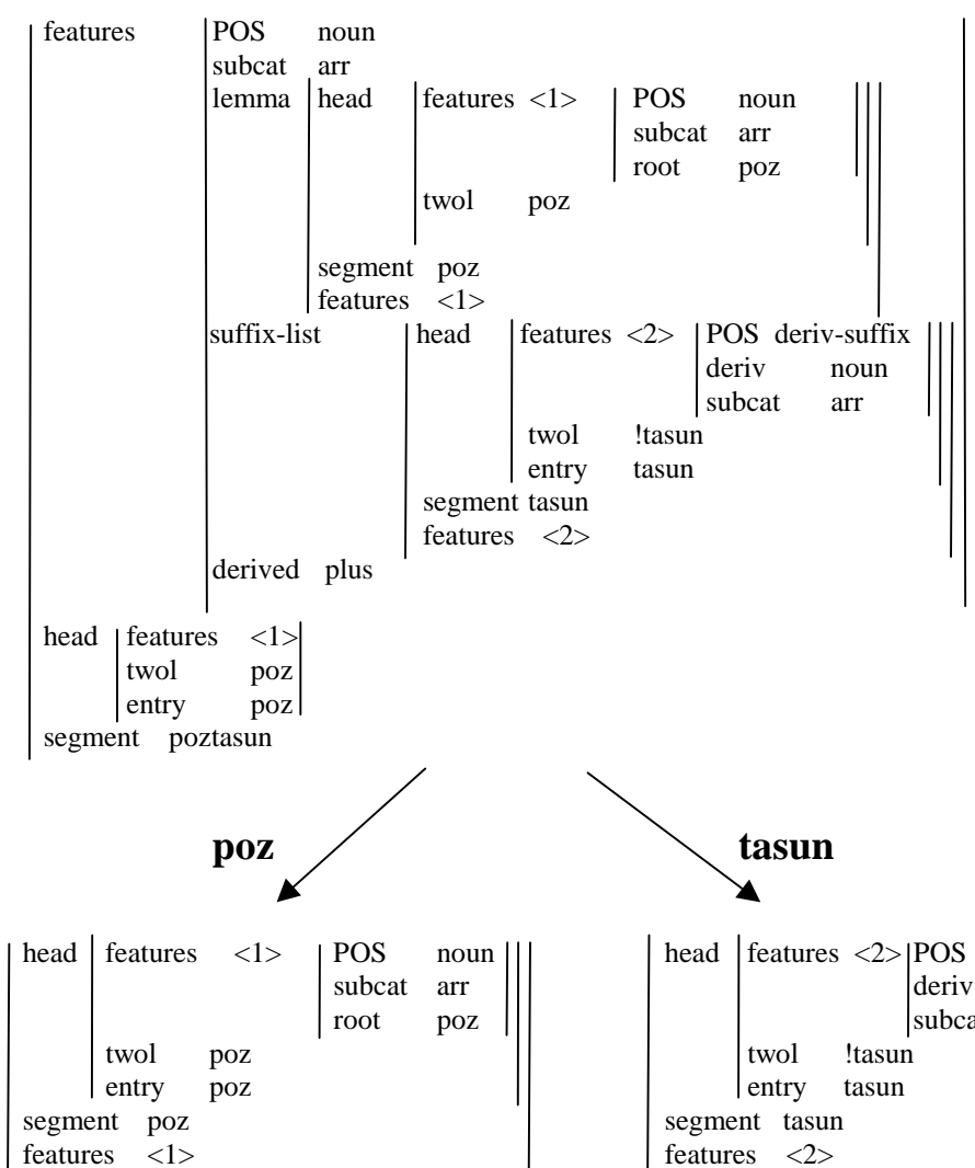
Figure 3: An example of complex morphological representation
