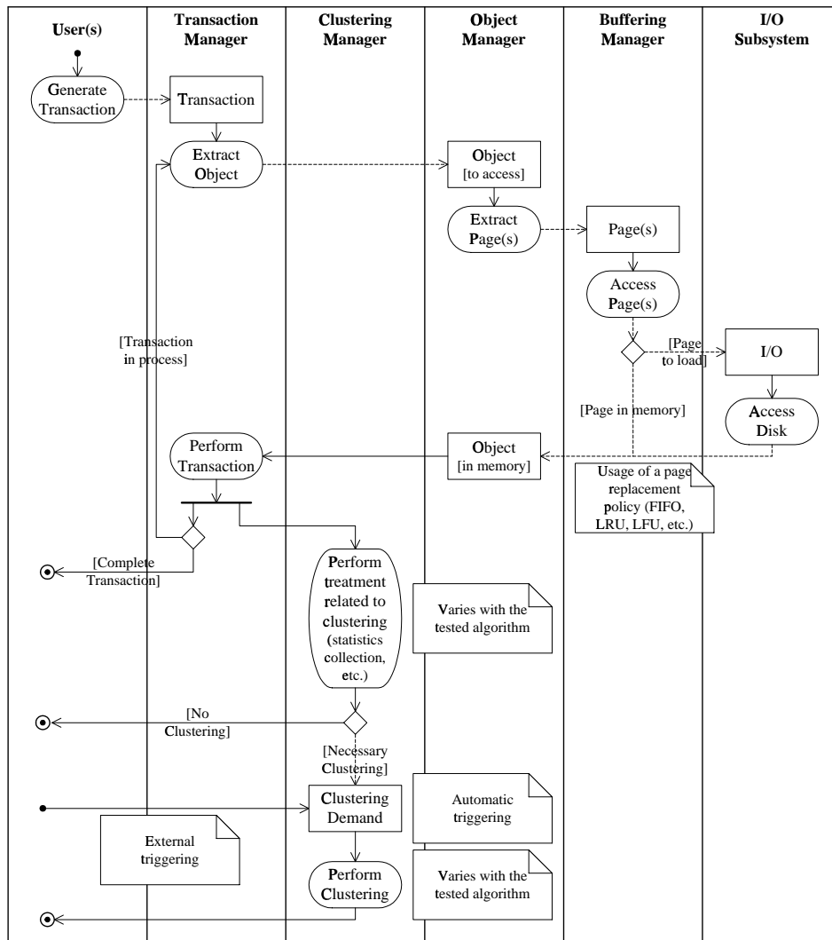
Figure 4: Knowledge model
