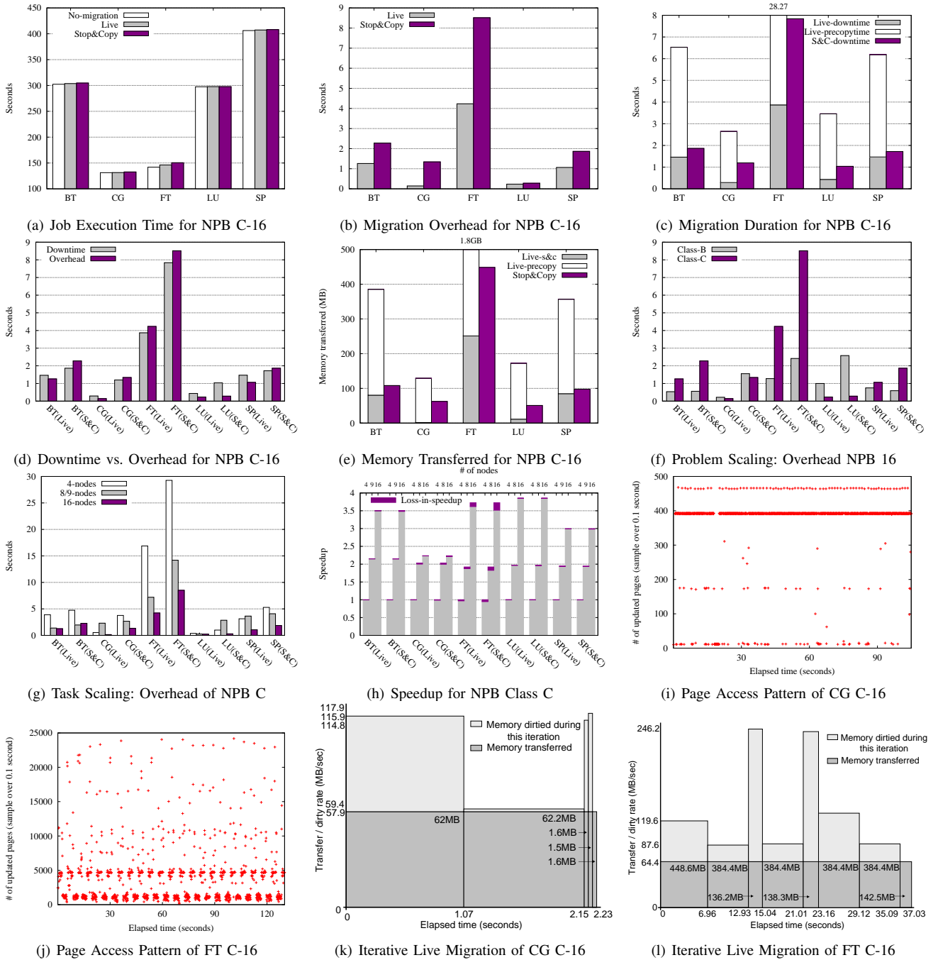
Fig. 4: Evaluation with NPB (C-16: Class C on 16 Nodes)
