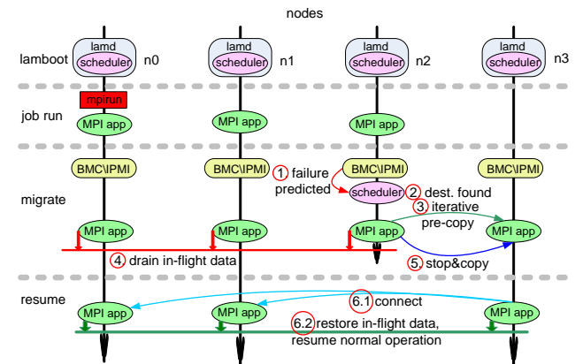
Fig. 1: Job Live Migration
