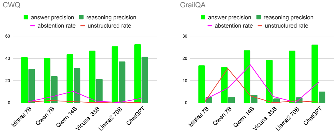
Figure 7: The precision of LLMs using few-shot CoT - SC prompt.
