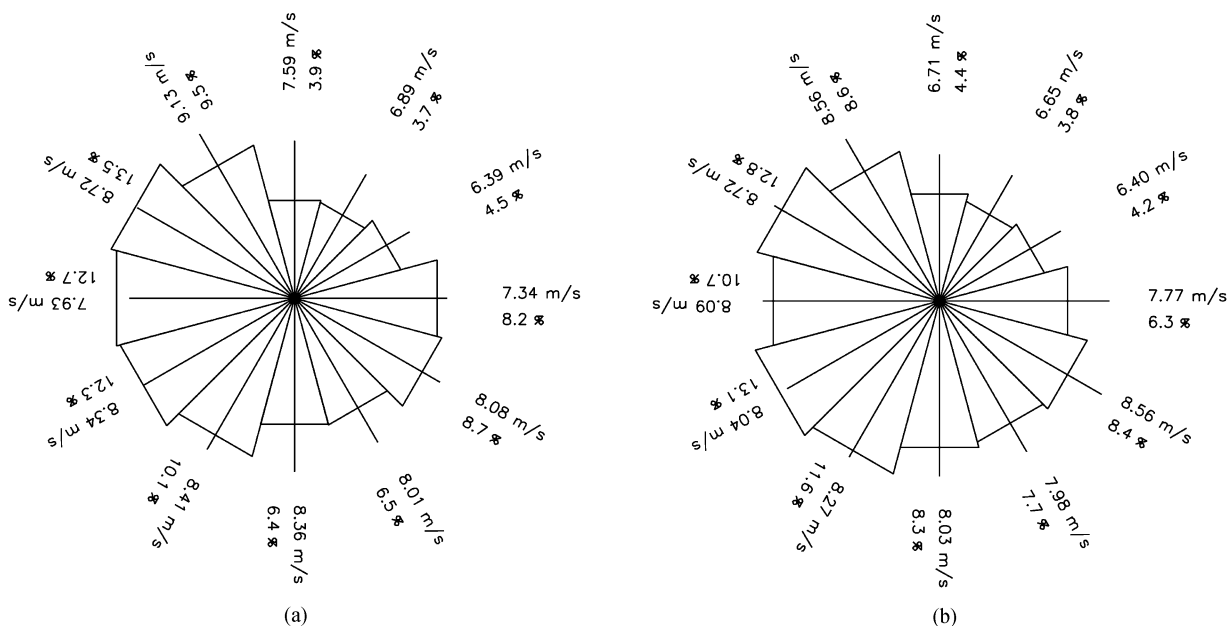
Fig. 13. Wind rose for Horns Rev based on (top) QuikSCAT (bottom) mast data.
