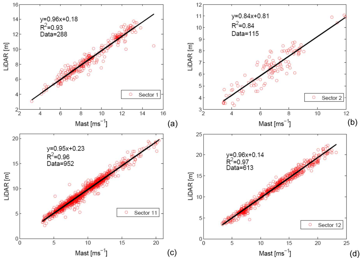
Fig. 2. Comparison of horizontal mean wind speeds observed from LiDAR at 63 m with cup anemometer measurements at 62 m AMSL in four 30^\circ sectors in the period May 3, 2006 to October 24, 2006. Data less than 2 \text{ ms}^{-1} are not included as well as rainy days.
