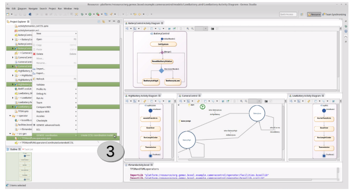
Fig. 3. Generation of the coordination specification for a surveillance camera system
