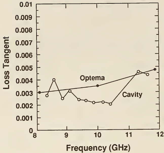
Figure 3.9: Imaginary part of permittivity for a barium titanate compound \circ \circ \circ -cavity and \dots - optimized solution.
