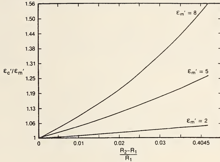
Figure C.3: The gap correction calculated for various values of \epsilon'_{mR} , where R_2, R_1 are the radii of the inner conductor and sample respectively.
