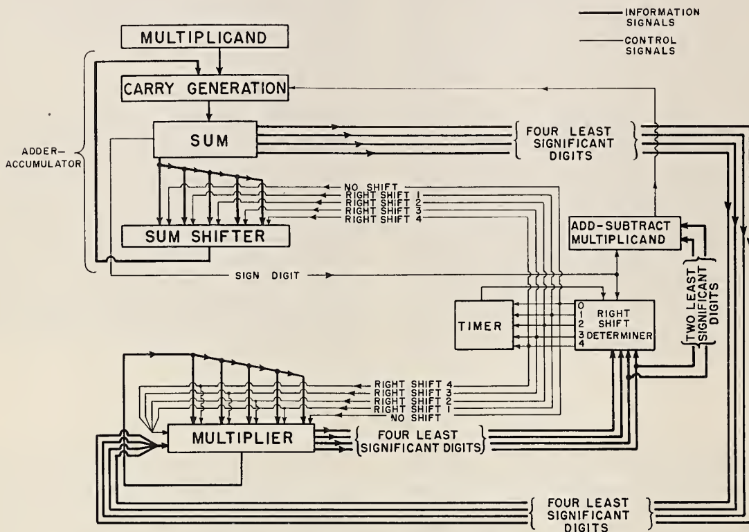
FIGURE 2.1. Schematic diagram for shortcut multiplier.
