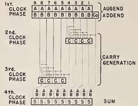
FIGURE 1.7. Nine-bit parallel binary adder.
