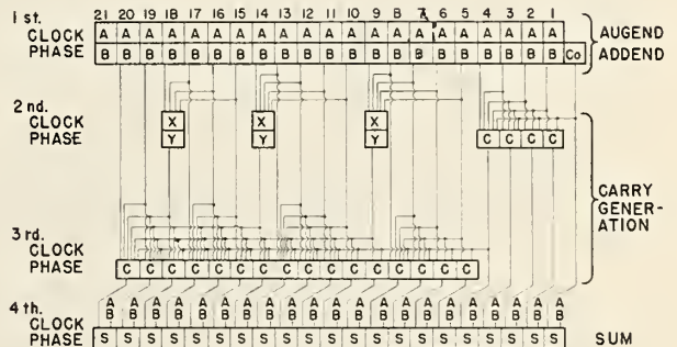
FIGURE 1.9. Twenty-one-bit parallel binary adder.
