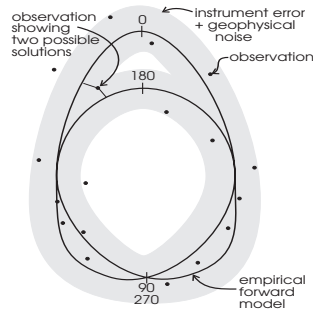
Figure 1: A two dimensional sketch of the scatterometer measurement space. The two dimensional slice is taken through the measurement manifold at constant wind speed. For a noisy observation there are at least two solutions in wind direction.
