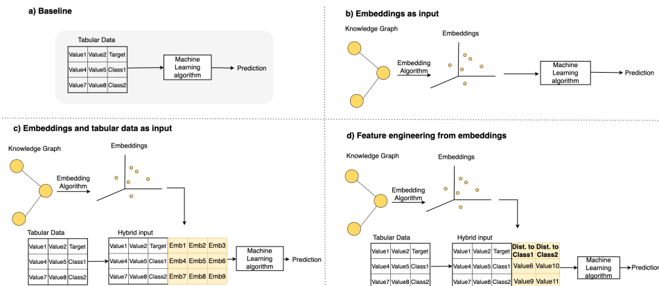
Figure 1: Approaches for medical diagnostic problem with variations of the input data: (a) Baseline method (without KG), (b) KG embeddings as direct inputs, (c) KG embeddings combined with tabular data, and (d) Feature engineering with distance metrics from KG embeddings.
