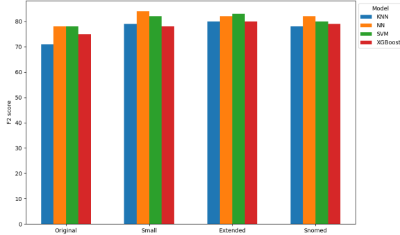
Figure 2: Average F2 Score for Different Models with no KG and Various KG-Modified Inputs.
