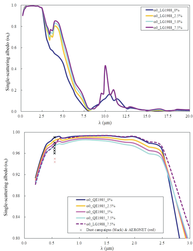
Figure 4. Spectral single-scattering albedo (SSA) for mixtures of illite and hematite with varying percentages and refractive indices at wavelengths of 0–20 \mu\text{m} (a) and 0–3 \mu\text{m} (b) with comparison to field observed results at 550 nm.
