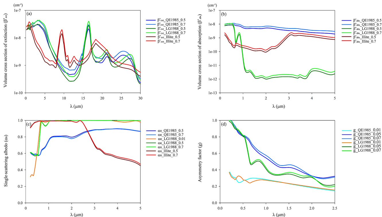
Figure 2. The calculated spectral optical properties for hematite, goethite and illite with different complex refractive index and size distribution. (a) Volume cross section of extinction, (b) volume cross section of absorption, (c) single-scattering albedo and (d) asymmetry factor.
