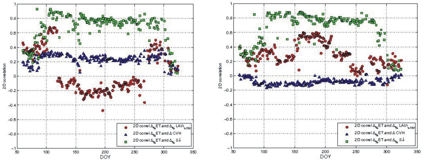
Fig. 8. Spatial (2-D) correlation over Europe between the ET mean relative bias (based on the images between 09:00 to 12:00 UTC) and model differences: (1) LAI/r_{s\ min} (red diamonds), (2) High vegetation percentage (CVH, blue triangles), and (3) S\downarrow mean relative bias (DSSF, green squares). At left: comparison between LSA SAF MET and ECMWF. At right: comparison between LSA SAF MET and GLDAS.
