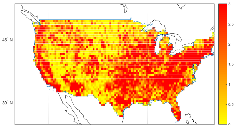
Figure 1. CPC gauge coverage during 2007–2012 expressed as average number of working rain gauges per day within each 0.25^\circ spatial grid cell.
