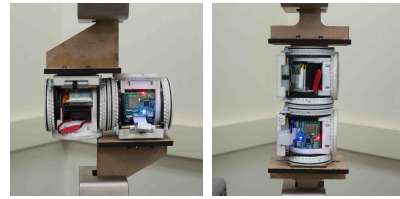
Fig. 7: (Left) Shear and (Right) Angular Offset test setups
