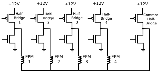
Fig. 6: Circuit for Driving EP Magnets.
