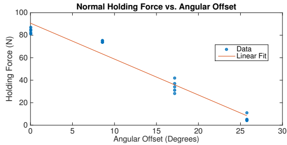
Fig. 12: Normal Holding Force vs. Angular Offset. Linear fit: y = -3.194x + 90.7
