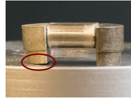
Fig. 5: Misaligned EP magnet. The left pole (circled in red) makes contact on its edge rather than its face, reducing contact surface area and flux transmission.
