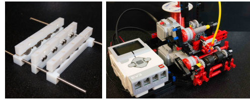
Fig. 4: Gluing fixture (left) and winding machine (right)
