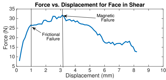
Fig. 11: Force vs. displacement in shear. Peak force of 31.8N at displacement of 3.1mm. Note while static friction failure appears to occur at a displacement of 1mm, this large displacement is due to deformation (slop) of the module, not movement of the magnets.
