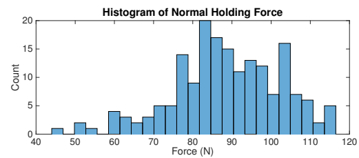
Fig. 9: Histogram of Holding Forces Under Normal Load. Mean=88.4N, Std=13.9N.
