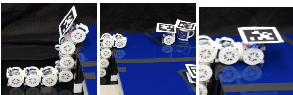
Fig. 14: Ledge exploration. (Left) Seven-module snake lifts its head to the top of a 3-module high ledge. (Center) Head module detaches, and explores the surface. (Right) Head module autonomously reattaches, and snake descends.
