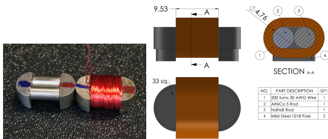
Fig. 3: Left: EP magnets, before and after winding. Right: Technical drawing of EP magnet, dimensions in millimeters.
