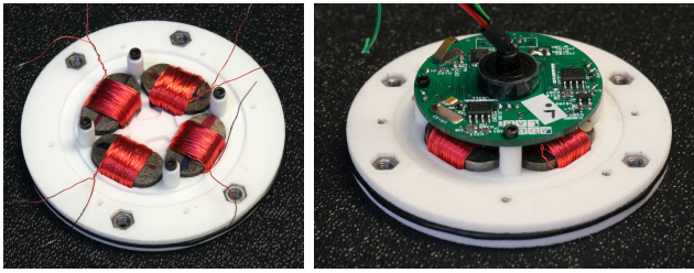
Fig. 1: Left: Internal view of magnets in EP-Face. Right: Internal view of EP-face with circuit board and slipping.
