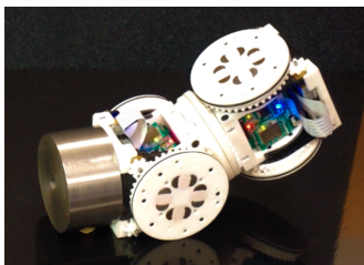
Fig. 15: SMORES-EP module moving a 1kg metal block while lifting another module in the air.
