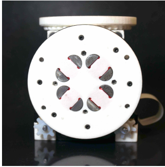
Fig. 2: EP-face on a SMORES-EP module.
