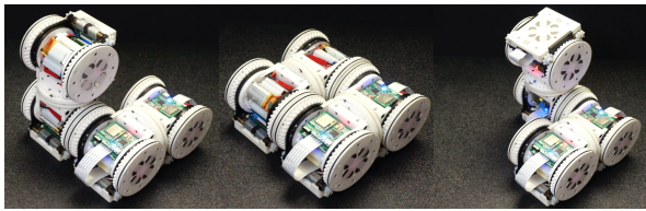
Fig. 13: Slide-by docking is made possible by the thin profile of the EP-Face.
