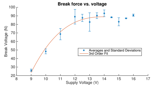
Fig. 10: Face Break Force vs. Supply Voltage. Cubic fit: y = 0.313x^3 - 14.3x^2 + 215x - 981
