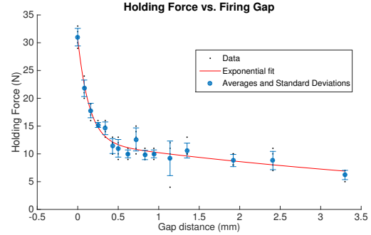
Fig. 8: Plot of Holding Force vs. Gap at Firing. Exponential fit: y = 18.63 \exp(-7.019x) + 12.08 \exp(-0.1697x)
