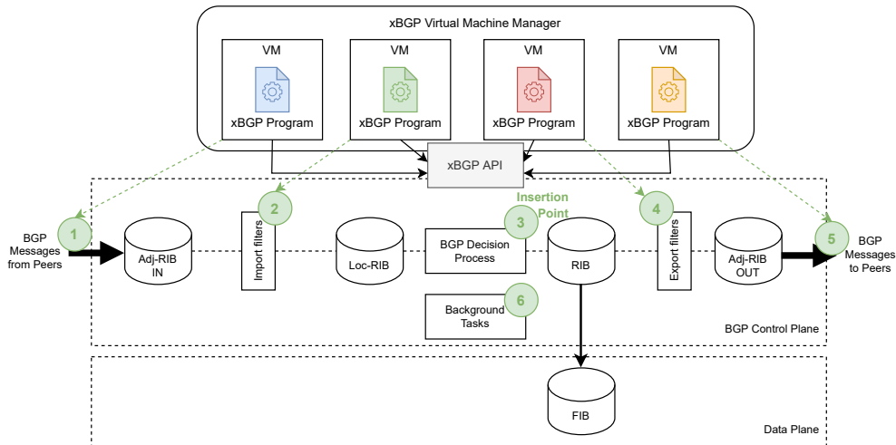
Figure 1: An xBGP compliant implementation exposes the abstract BGP data structures defined in RFC4271 through a generic API and uses libxBGP 's Virtual Machine Manager to attach the bytecode that implements extensions to specific insertion points (green circles). The four bytecodes in this example support a simple GeoLoc BGP attribute. For each xBGP program, we provide the set of helper functions used to retrieve data from the host implementation.
