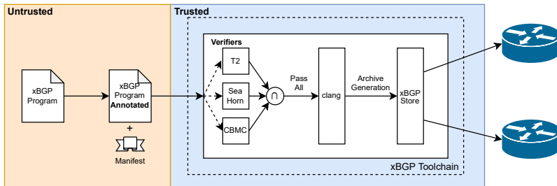
Figure 2: High-level view of the xBGP verification toolchain.
