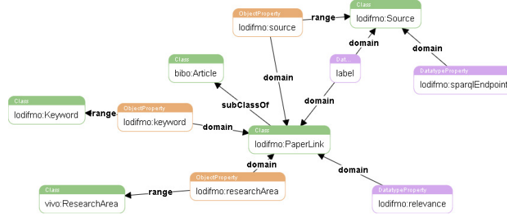
Fig. 1. Ontology model of scientific portal (Fragment)
