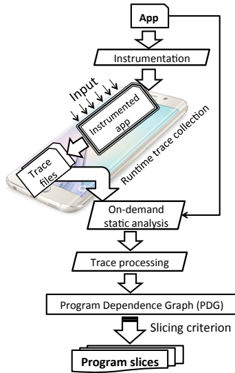
Fig. 4: AndroidSlicer overview.
