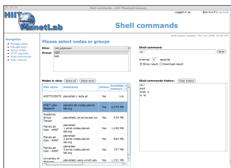
Shell command execution
